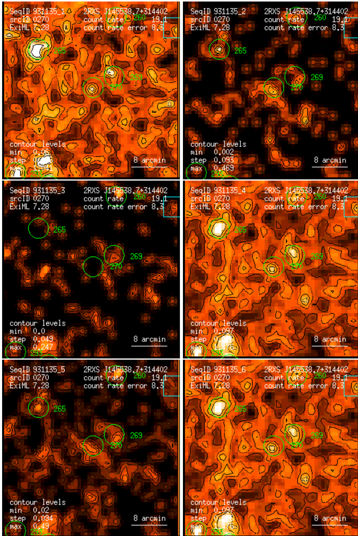
Figure 270: RASS 931135: detection 0270: band rate images, Gaussian filter: (1) PSPC channels 11 – 41, (2) 52 – 90, (3) 91 – 201, (4) 11 – 235, (5) 52 – 201, (6) 11 – 201. Broad band rates in counts/ks. Band rate contour levels in counts/ks/arcmin 2 .
