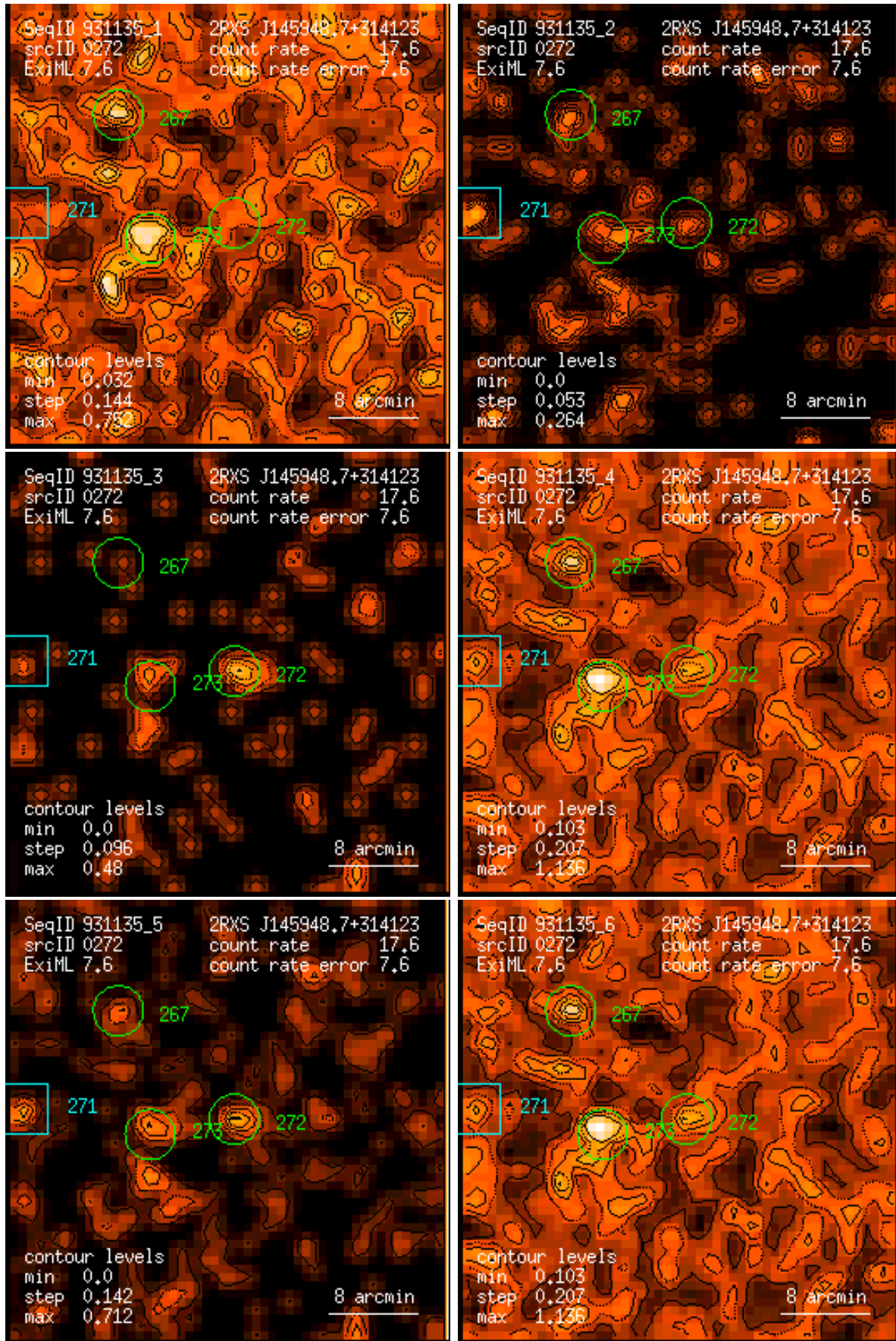
Figure 272: RASS 931135: detection 0272: band rate images, Gaussian filter: (1) PSPC channels 11 – 41, (2) 52 – 90, (3) 91 – 201, (4) 11 – 235, (5) 52 – 201, (6) 11 – 201. Broad band rates in counts/ks. Band rate contour levels in counts/ks/arcmin 2 .
