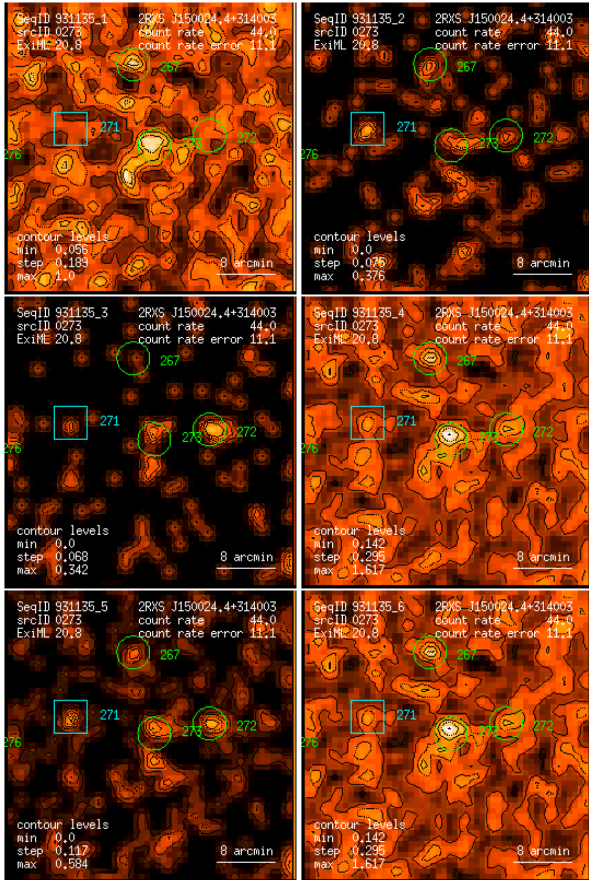
Figure 273: RASS 931135: detection 0273: band rate images, Gaussian filter: (1) PSPC channels 11 – 41, (2) 52 – 90, (3) 91 – 201, (4) 11 – 235, (5) 52 – 201, (6) 11 – 201. Broad band rates in counts/ks. Band rate contour levels in counts/ks/arcmin 2 .
