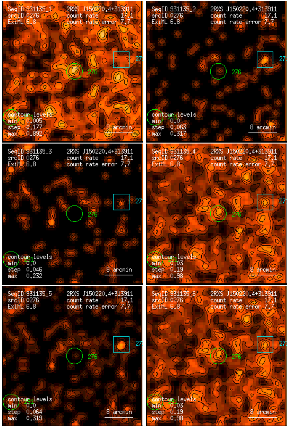
Figure 276: RASS 931135: detection 0276: band rate images, Gaussian filter: (1) PSPC channels 11 – 41, (2) 52 – 90, (3) 91 – 201, (4) 11 – 235, (5) 52 – 201, (6) 11 – 201. Broad band rates in counts/ks. Band rate contour levels in counts/ks/arcmin 2 .
