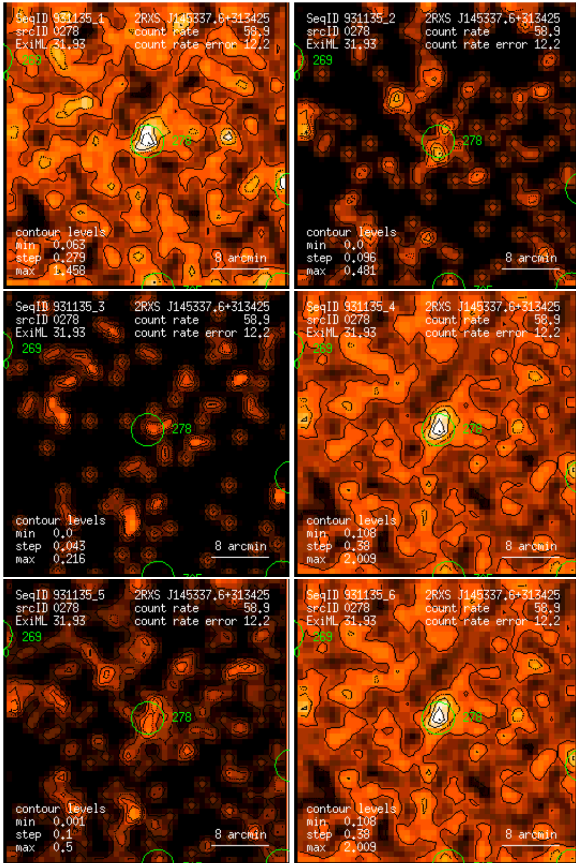
Figure 278: RASS 931135: detection 0278: band rate images, Gaussian filter: (1) PSPC channels 11 – 41, (2) 52 – 90, (3) 91 – 201, (4) 11 – 235, (5) 52 – 201, (6) 11 – 201. Broad band rates in counts/ks. Band rate contour levels in counts/ks/arcmin 2 .
