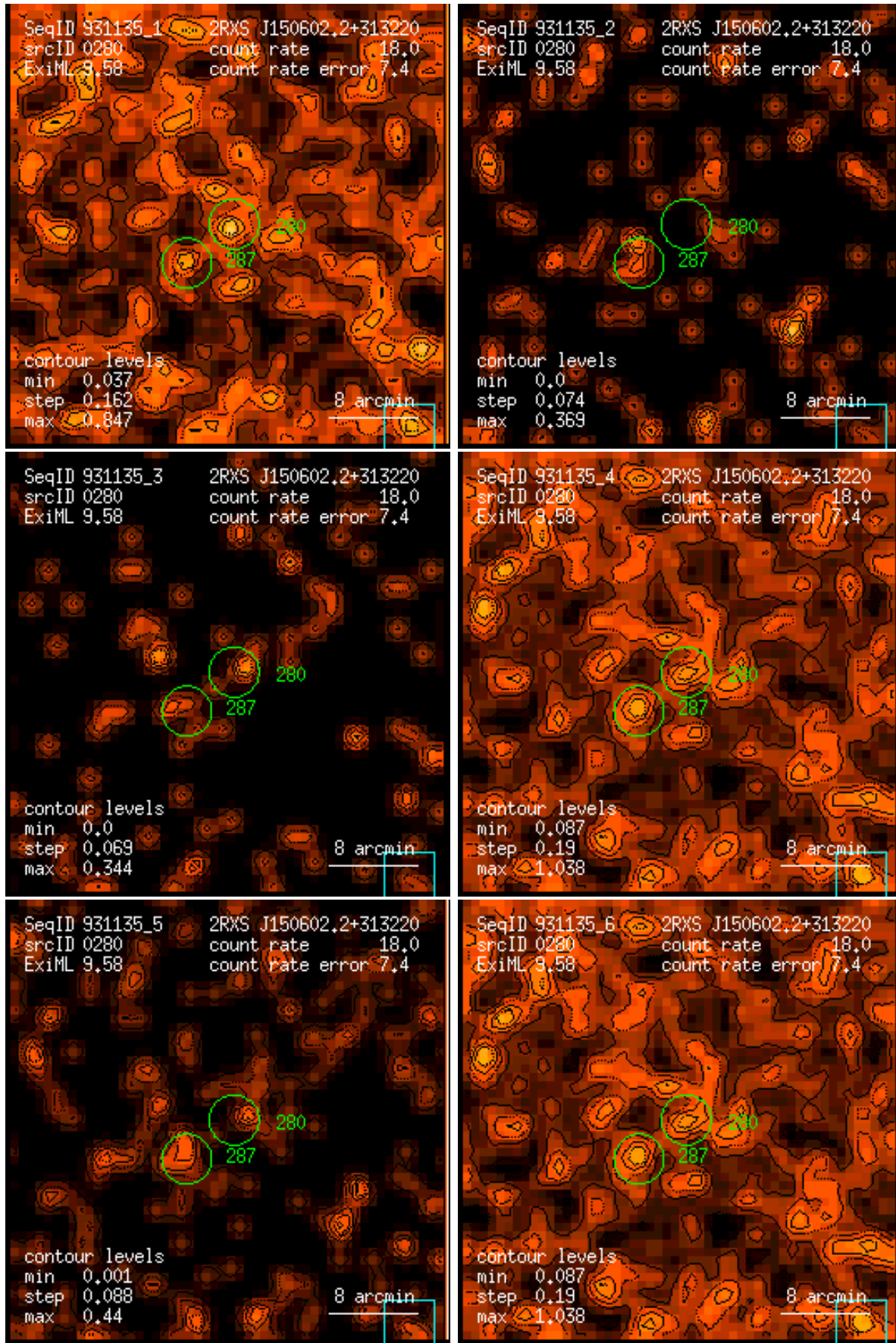
Figure 280: RASS 931135: detection 0280: band rate images, Gaussian filter: (1) PSPC channels 11 – 41, (2) 52 – 90, (3) 91 – 201, (4) 11 – 235, (5) 52 – 201, (6) 11 – 201. Broad band rates in counts/ks. Band rate contour levels in counts/ks/arcmin 2 .
