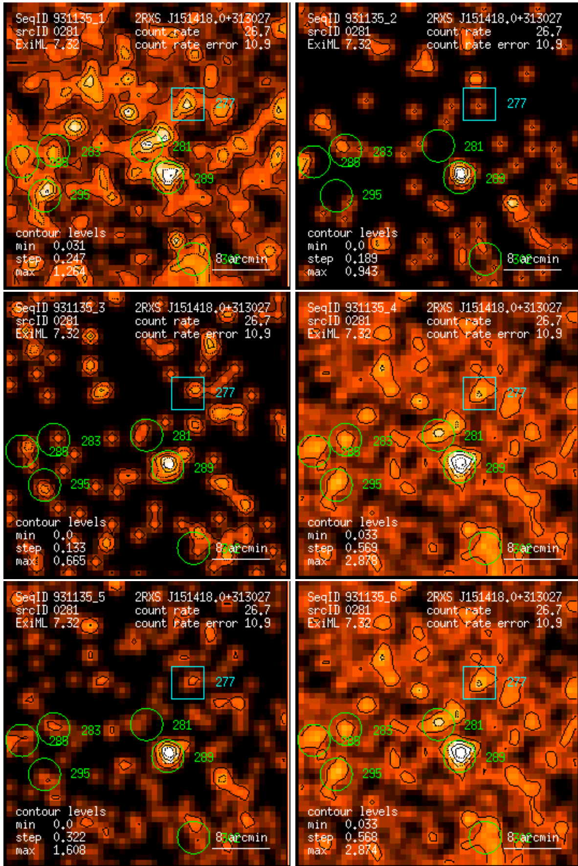
Figure 281: RASS 931135: detection 0281: band rate images, Gaussian filter: (1) PSPC channels 11 – 41, (2) 52 – 90, (3) 91 – 201, (4) 11 – 235, (5) 52 – 201, (6) 11 – 201. Broad band rates in counts/ks. Band rate contour levels in counts/ks/arcmin 2 .
