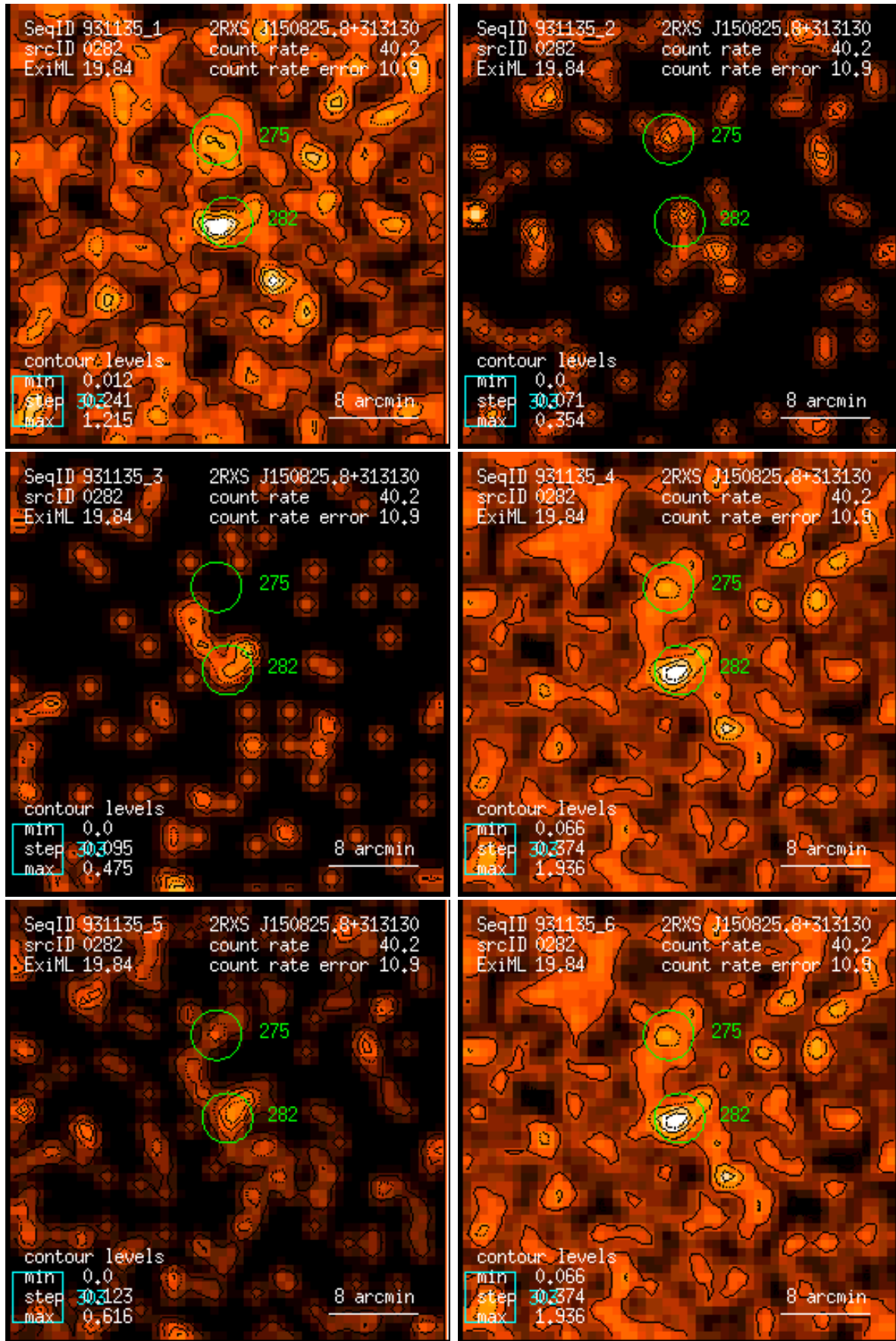
Figure 282: RASS 931135: detection 0282: band rate images, Gaussian filter: (1) PSPC channels 11 – 41, (2) 52 – 90, (3) 91 – 201, (4) 11 – 235, (5) 52 – 201, (6) 11 – 201. Broad band rates in counts/ks. Band rate contour levels in counts/ks/arcmin 2 .
