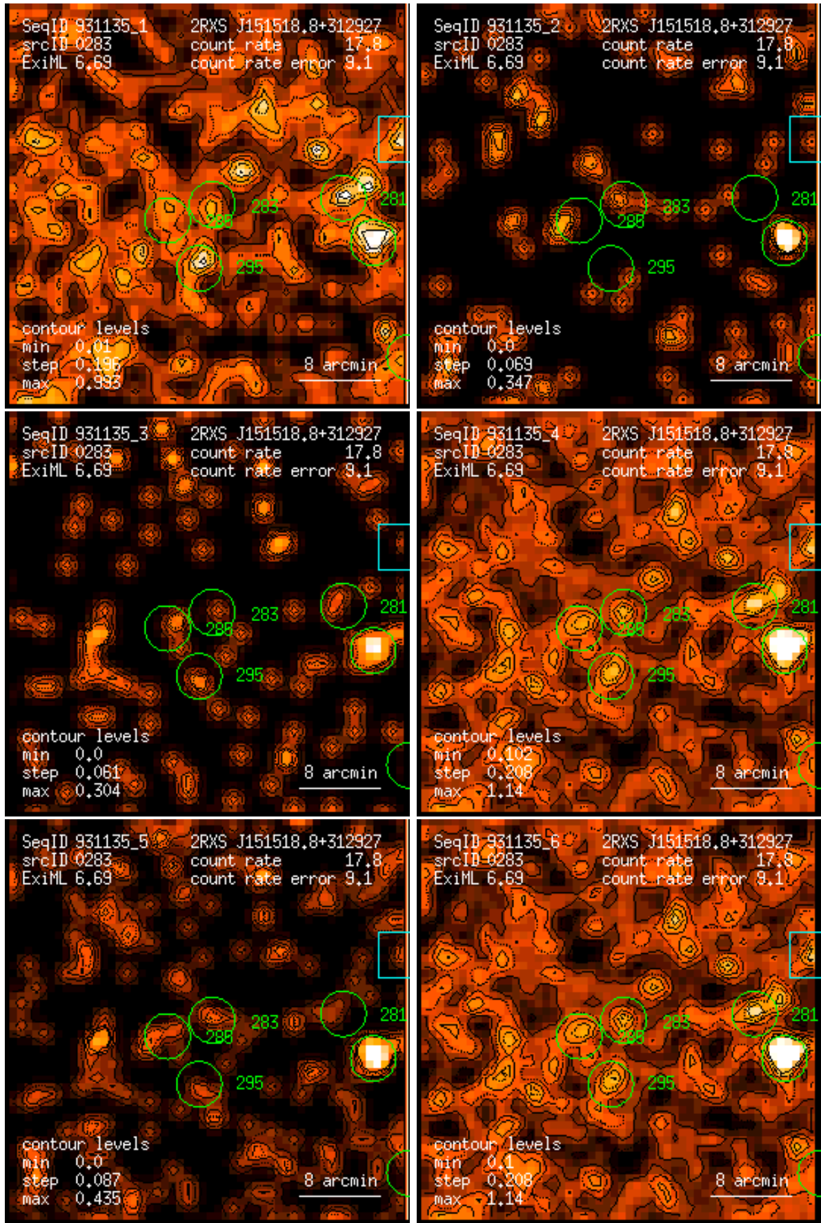
Figure 283: RASS 931135: detection 0283: band rate images, Gaussian filter: (1) PSPC channels 11 – 41, (2) 52 – 90, (3) 91 – 201, (4) 11 – 235, (5) 52 – 201, (6) 11 – 201. Broad band rates in counts/ks. Band rate contour levels in counts/ks/arcmin 2 .
