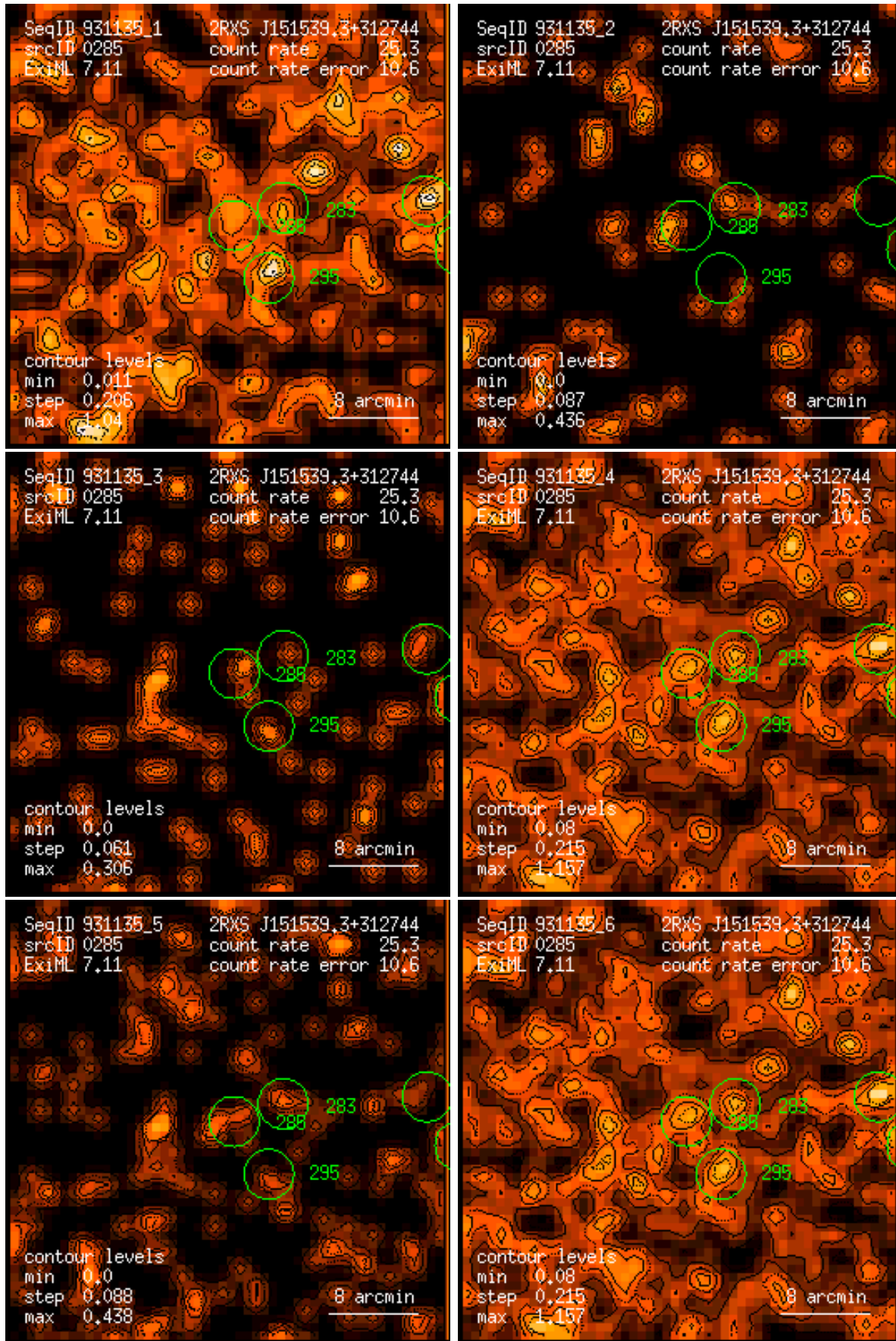
Figure 285: RASS 931135: detection 0285: band rate images, Gaussian filter: (1) PSPC channels 11 – 41, (2) 52 – 90, (3) 91 – 201, (4) 11 – 235, (5) 52 – 201, (6) 11 – 201. Broad band rates in counts/ks. Band rate contour levels in counts/ks/arcmin 2 .
