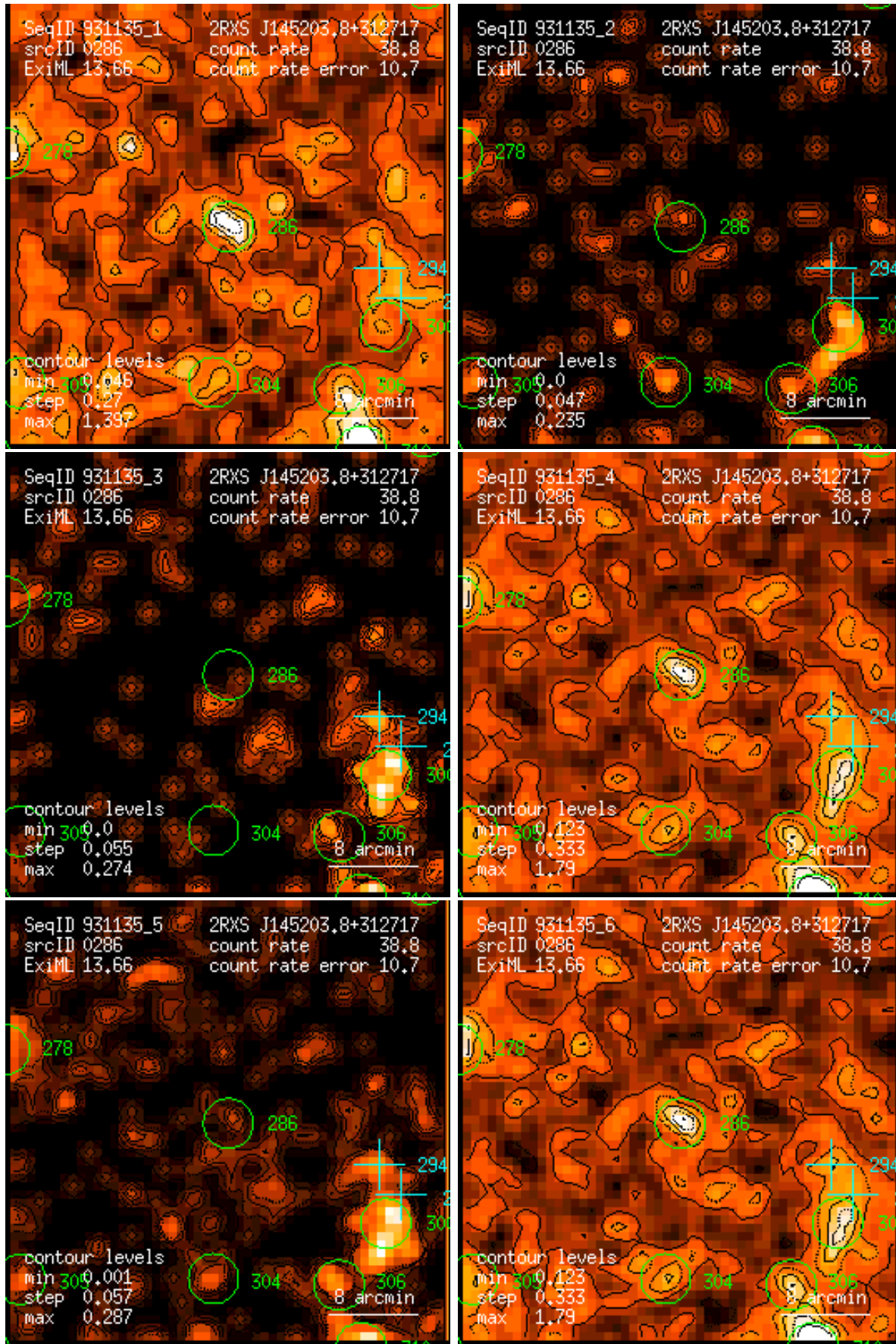
Figure 286: RASS 931135: detection 0286: band rate images, Gaussian filter: (1) PSPC channels 11 – 41, (2) 52 – 90, (3) 91 – 201, (4) 11 – 235, (5) 52 – 201, (6) 11 – 201. Broad band rates in counts/ks. Band rate contour levels in counts/ks/arcmin 2 .
