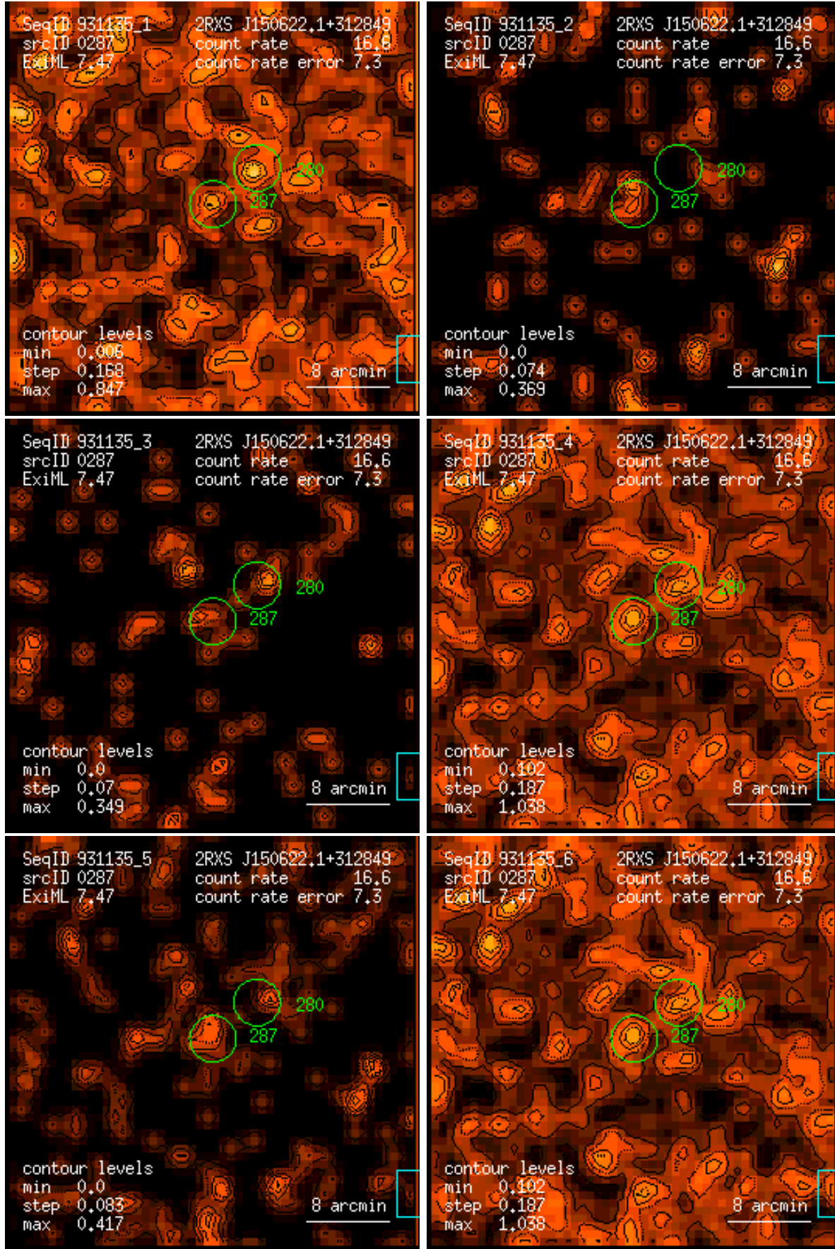
Figure 287: RASS 931135: detection 0287: band rate images, Gaussian filter: (1) PSPC channels 11 – 41, (2) 52 – 90, (3) 91 – 201, (4) 11 – 235, (5) 52 – 201, (6) 11 – 201. Broad band rates in counts/ks. Band rate contour levels in counts/ks/arcmin 2 .
