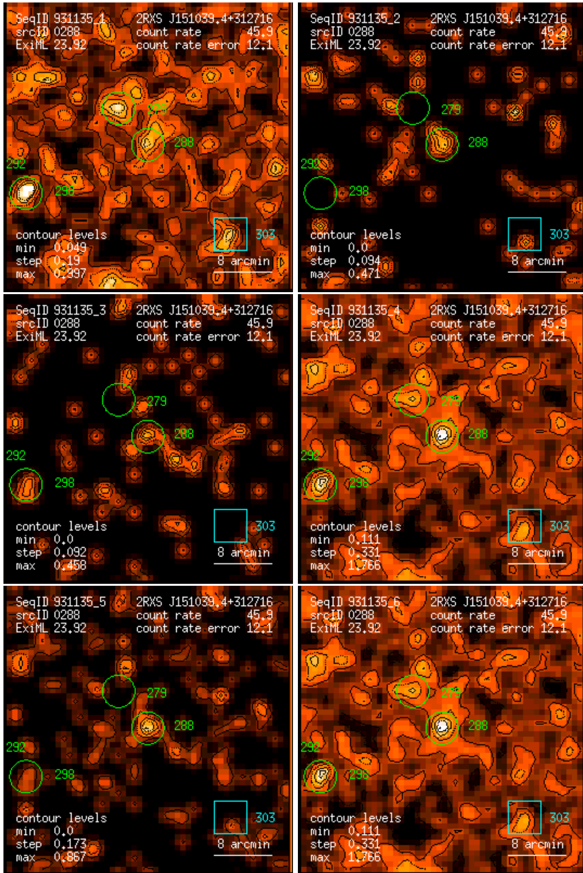
Figure 288: RASS 931135: detection 0288: band rate images, Gaussian filter: (1) PSPC channels 11 – 41, (2) 52 – 90, (3) 91 – 201, (4) 11 – 235, (5) 52 – 201, (6) 11 – 201. Broad band rates in counts/ks. Band rate contour levels in counts/ks/arcmin 2 .
