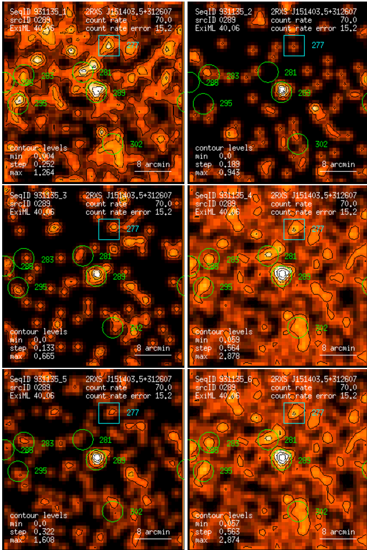
Figure 289: RASS 931135: detection 0289: band rate images, Gaussian filter: (1) PSPC channels 11 – 41, (2) 52 – 90, (3) 91 – 201, (4) 11 – 235, (5) 52 – 201, (6) 11 – 201. Broad band rates in counts/ks. Band rate contour levels in counts/ks/arcmin 2 .
