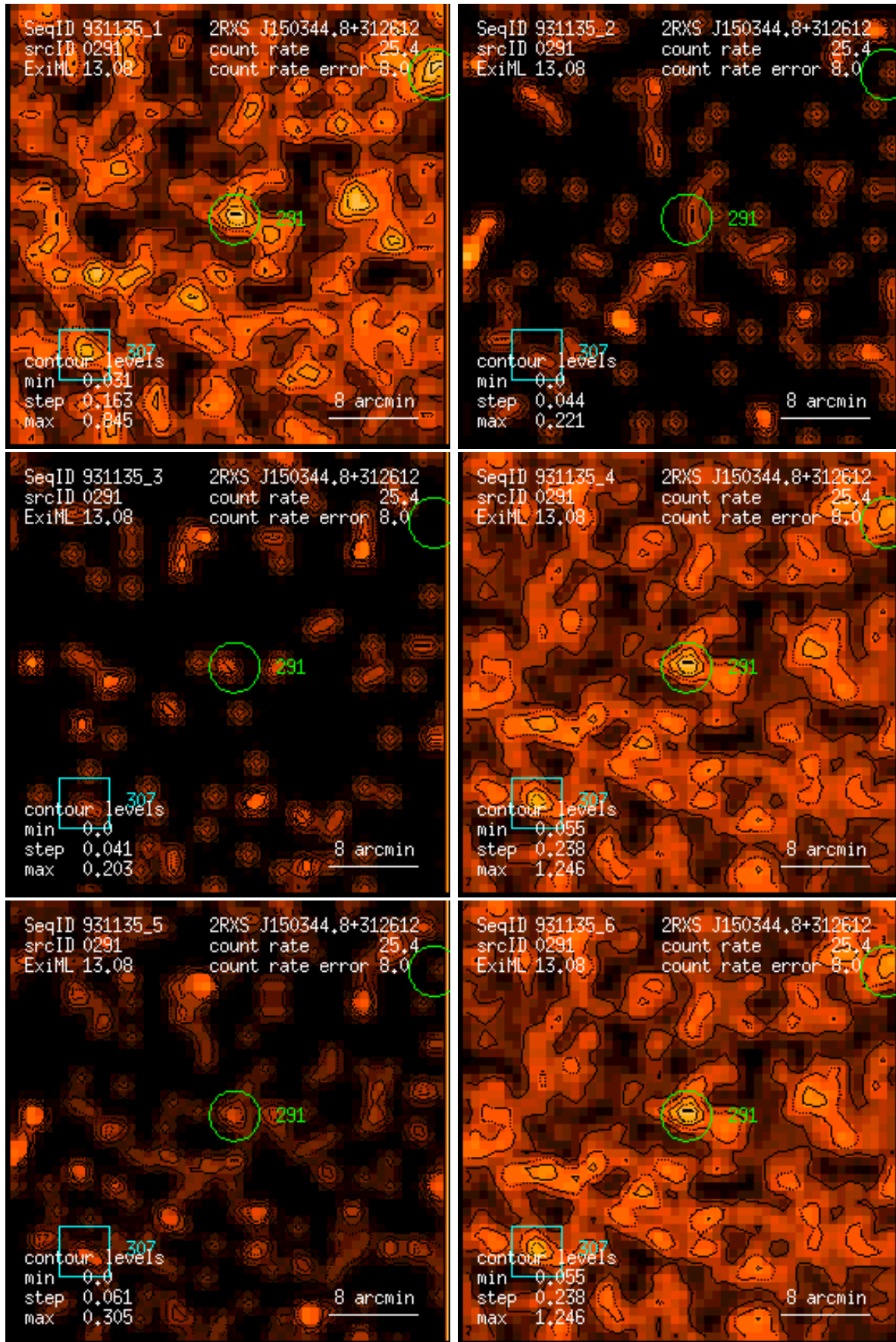
Figure 291: RASS 931135: detection 0291: band rate images, Gaussian filter: (1) PSPC channels 11 – 41, (2) 52 – 90, (3) 91 – 201, (4) 11 – 235, (5) 52 – 201, (6) 11 – 201. Broad band rates in counts/ks. Band rate contour levels in counts/ks/arcmin 2 .
