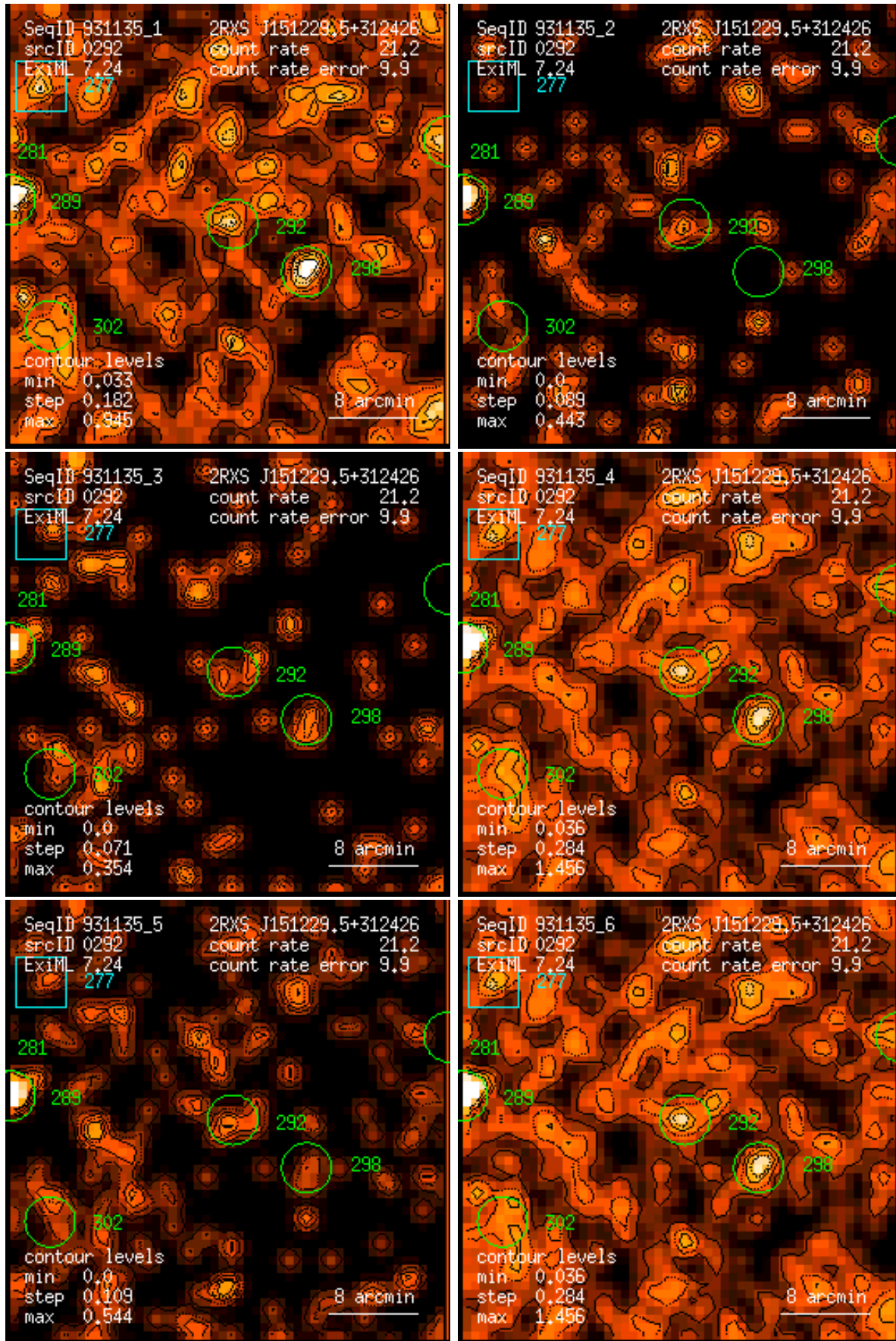
Figure 292: RASS 931135: detection 0292: band rate images, Gaussian filter: (1) PSPC channels 11 – 41, (2) 52 – 90, (3) 91 – 201, (4) 11 – 235, (5) 52 – 201, (6) 11 – 201. Broad band rates in counts/ks. Band rate contour levels in counts/ks/arcmin 2 .
