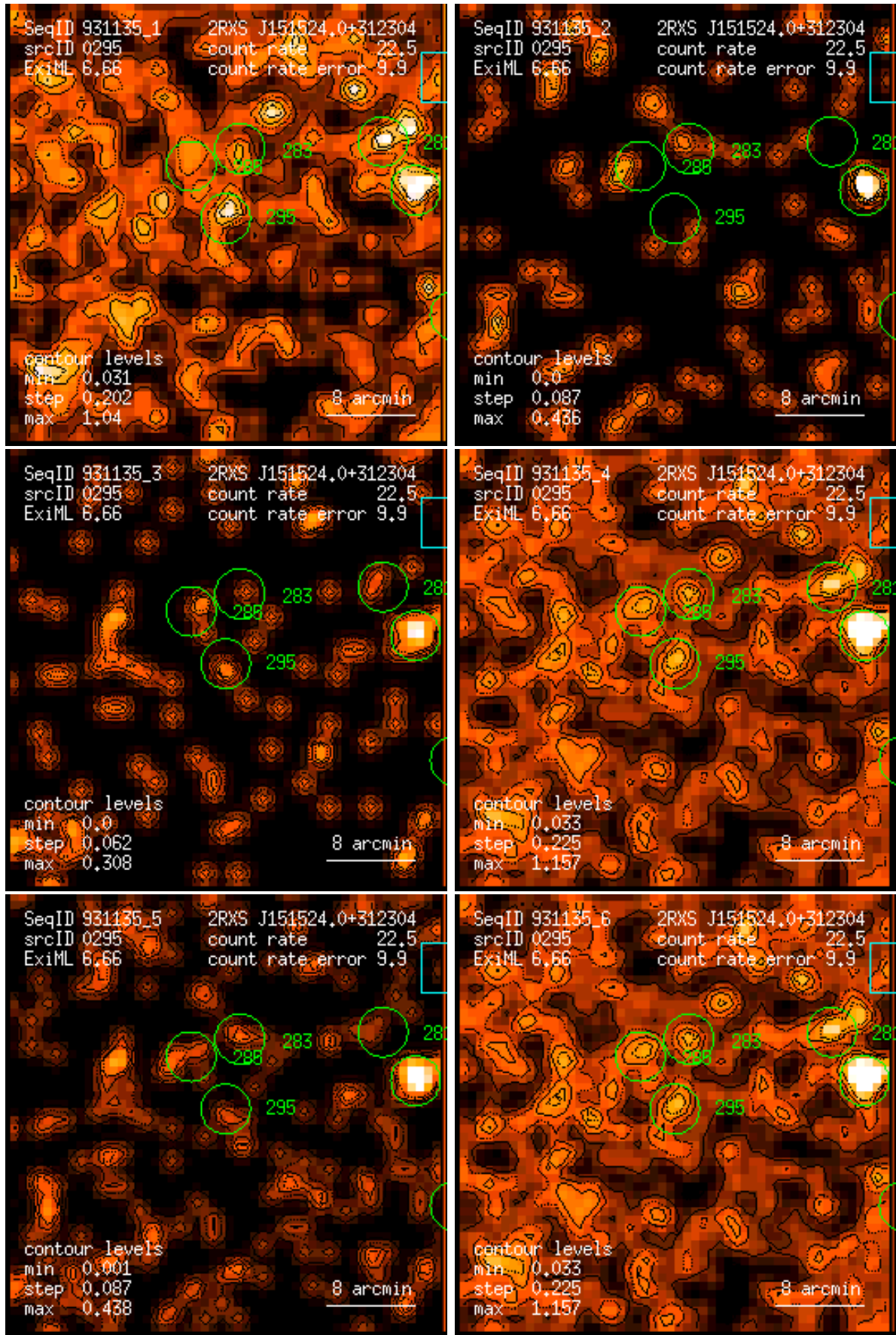
Figure 295: RASS 931135: detection 0295: band rate images, Gaussian filter: (1) PSPC channels 11 – 41, (2) 52 – 90, (3) 91 – 201, (4) 11 – 235, (5) 52 – 201, (6) 11 – 201. Broad band rates in counts/ks. Band rate contour levels in counts/ks/arcmin 2 .
