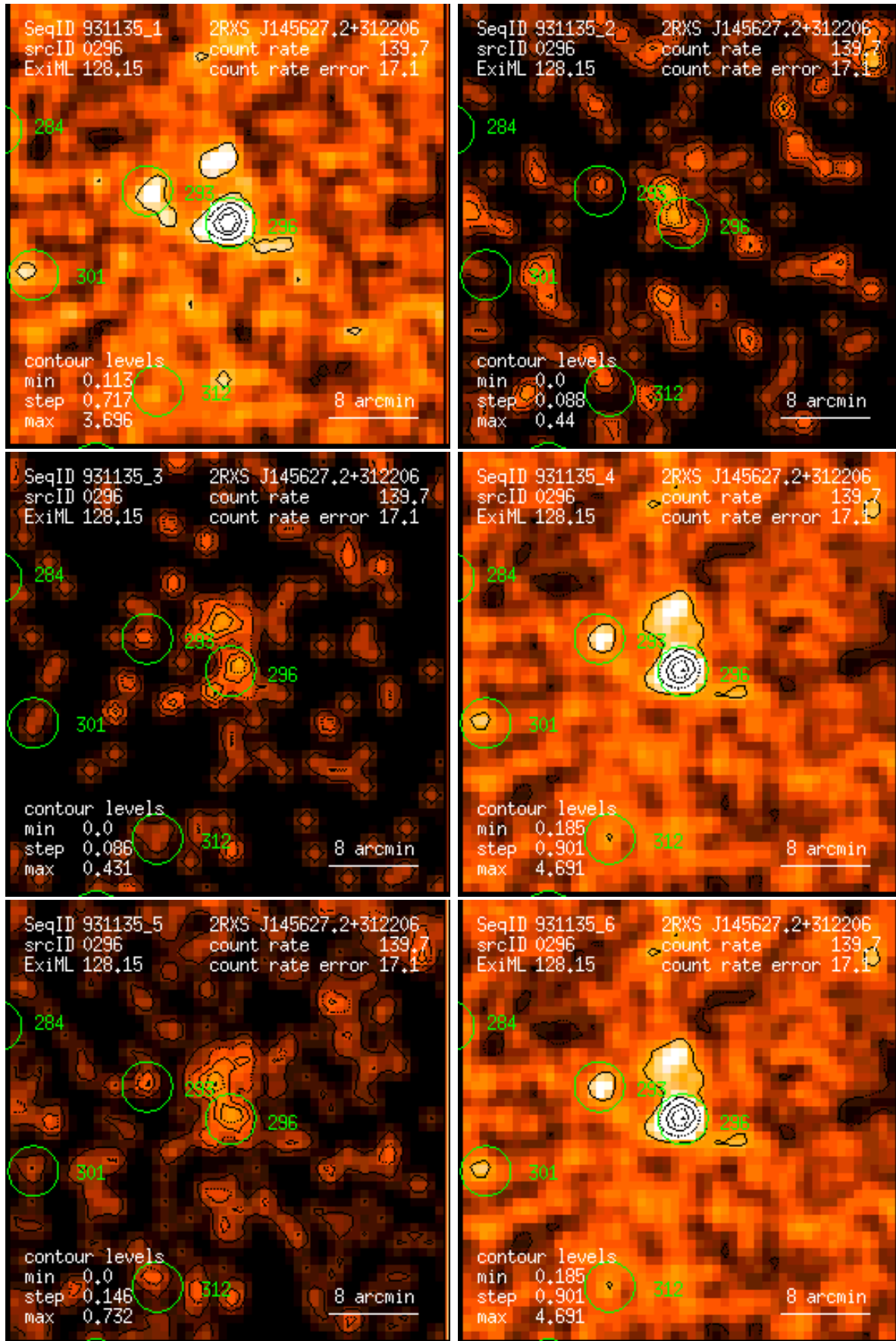
Figure 296: RASS 931135: detection 0296: band rate images, Gaussian filter: (1) PSPC channels 11 – 41, (2) 52 – 90, (3) 91 – 201, (4) 11 – 235, (5) 52 – 201, (6) 11 – 201. Broad band rates in counts/ks. Band rate contour levels in counts/ks/arcmin 2 .
