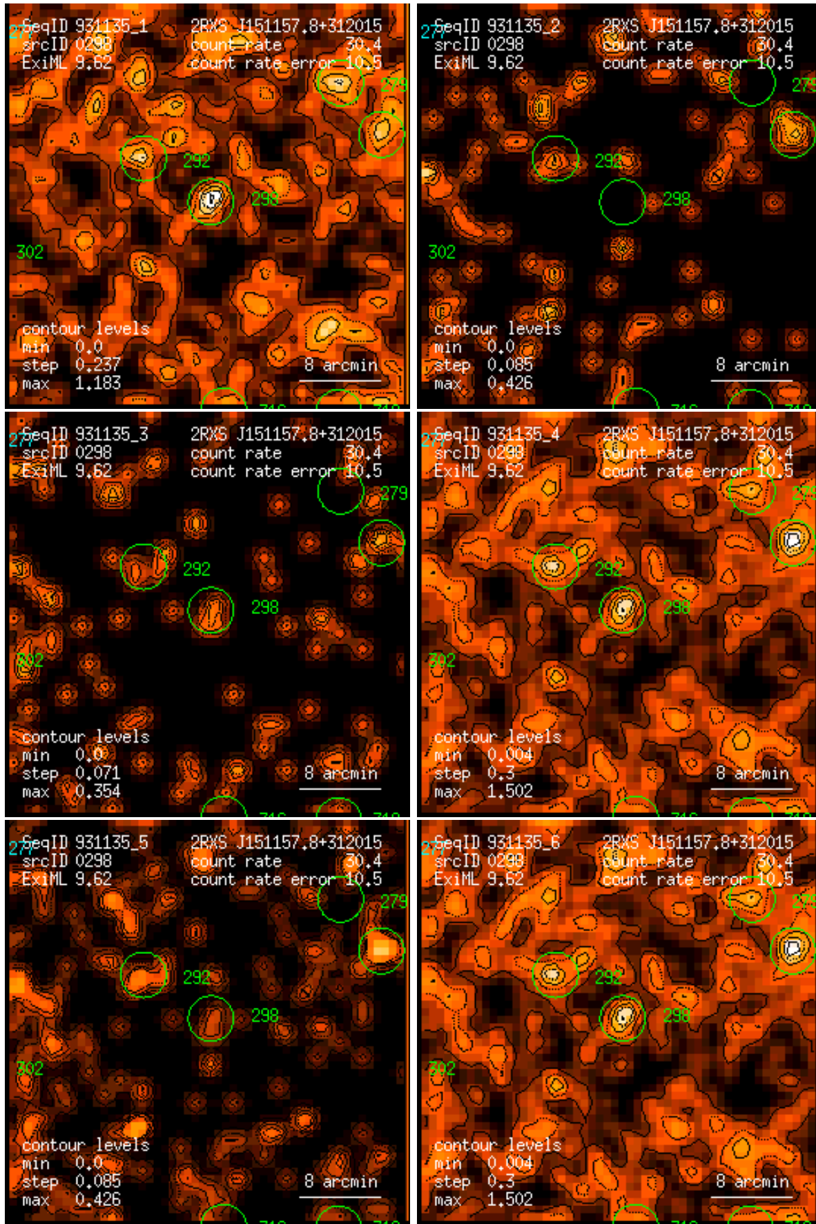
Figure 298: RASS 931135: detection 0298: band rate images, Gaussian filter: (1) PSPC channels 11 – 41, (2) 52 – 90, (3) 91 – 201, (4) 11 – 235, (5) 52 – 201, (6) 11 – 201. Broad band rates in counts/ks. Band rate contour levels in counts/ks/arcmin 2 .
