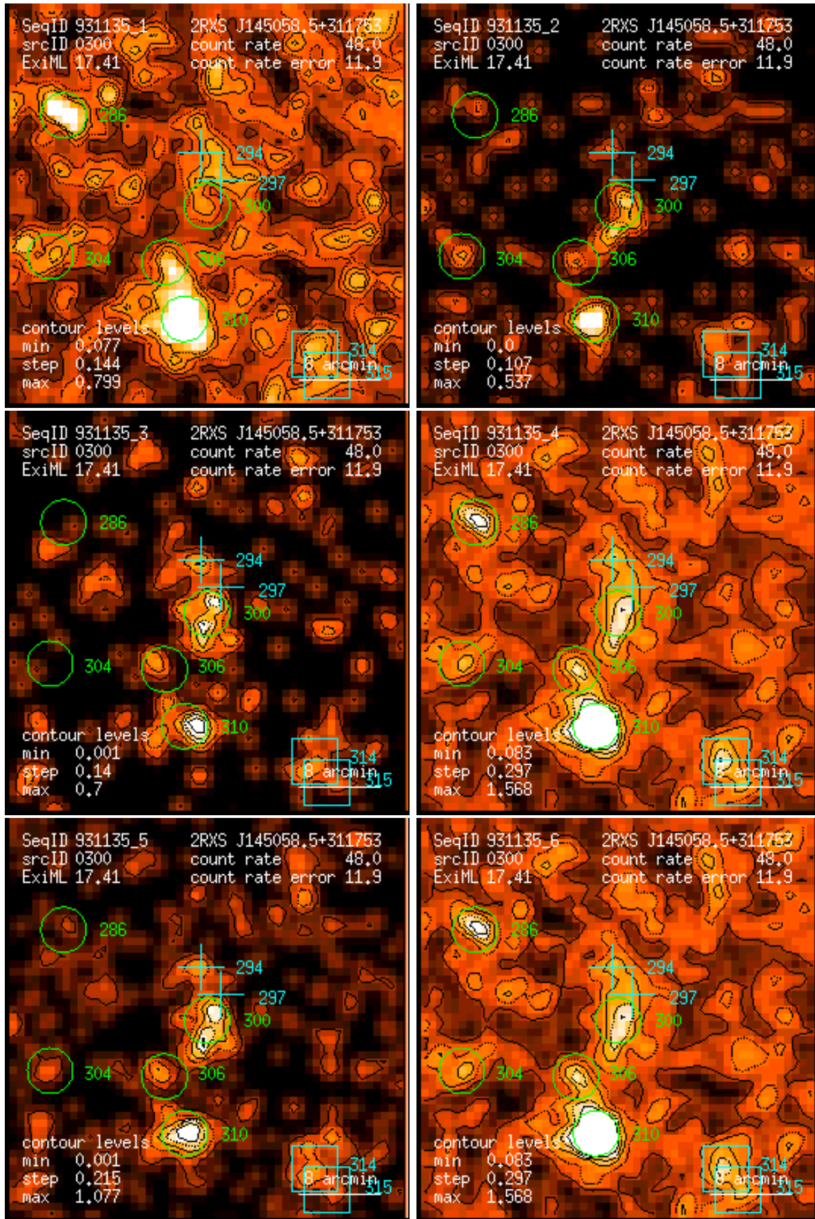
Figure 300: RASS 931135: detection 0300: band rate images, Gaussian filter: (1) PSPC channels 11 – 41, (2) 52 – 90, (3) 91 – 201, (4) 11 – 235, (5) 52 – 201, (6) 11 – 201. Broad band rates in counts/ks. Band rate contour levels in counts/ks/arcmin 2 .
