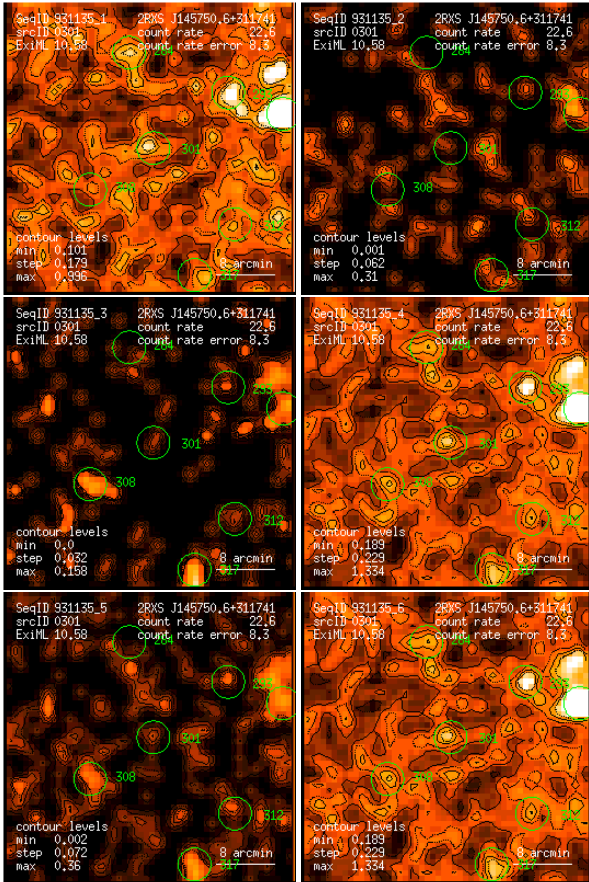
Figure 301: RASS 931135: detection 0301: band rate images, Gaussian filter: (1) PSPC channels 11 – 41, (2) 52 – 90, (3) 91 – 201, (4) 11 – 235, (5) 52 – 201, (6) 11 – 201. Broad band rates in counts/ks. Band rate contour levels in counts/ks/arcmin 2 .
