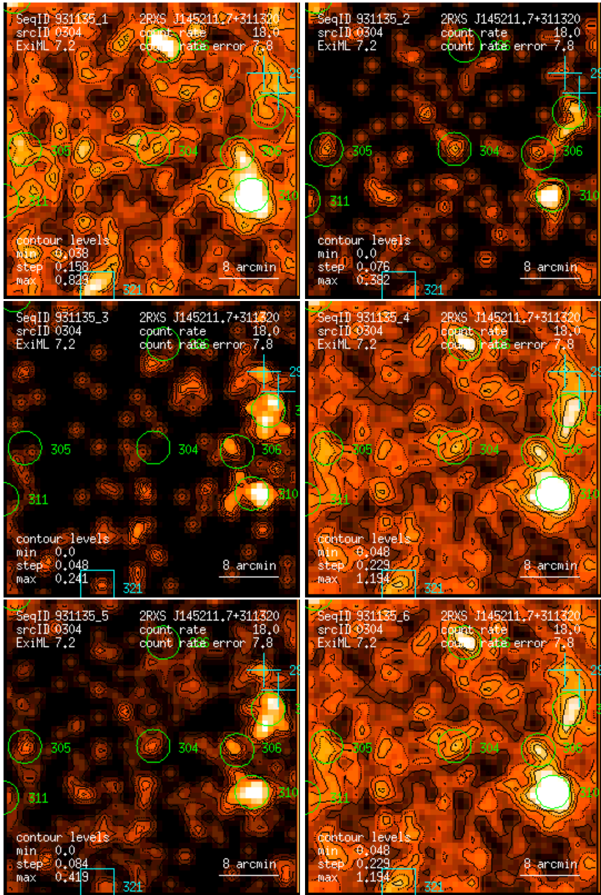
Figure 304: RASS 931135: detection 0304: band rate images, Gaussian filter: (1) PSPC channels 11 – 41, (2) 52 – 90, (3) 91 – 201, (4) 11 – 235, (5) 52 – 201, (6) 11 – 201. Broad band rates in counts/ks. Band rate contour levels in counts/ks/arcmin 2 .
