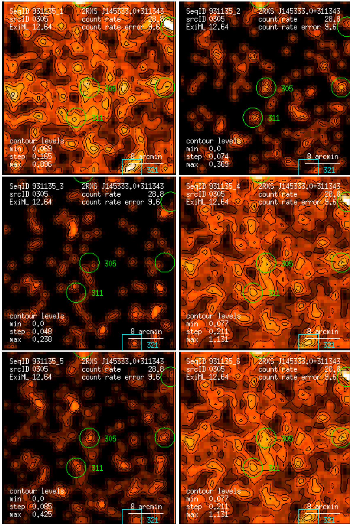
Figure 305: RASS 931135: detection 0305: band rate images, Gaussian filter: (1) PSPC channels 11 – 41, (2) 52 – 90, (3) 91 – 201, (4) 11 – 235, (5) 52 – 201, (6) 11 – 201. Broad band rates in counts/ks. Band rate contour levels in counts/ks/arcmin 2 .
