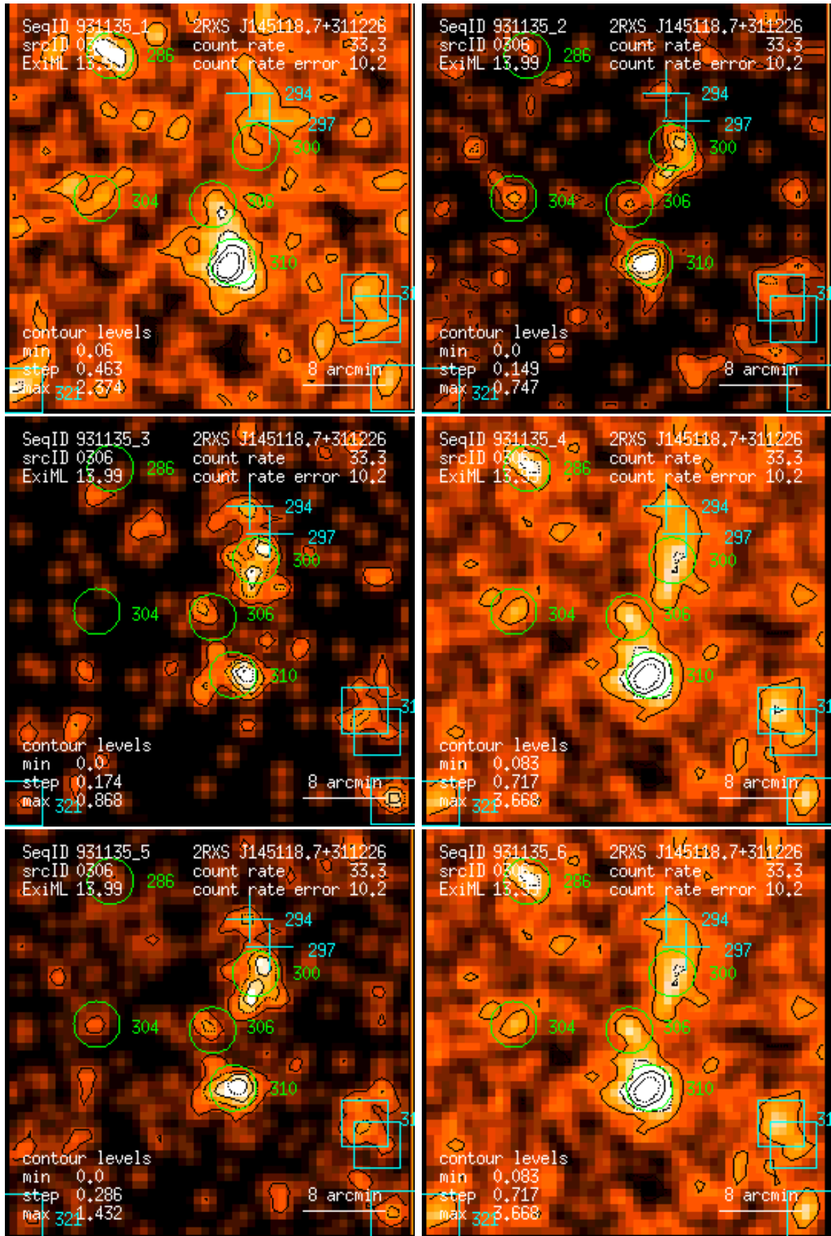
Figure 306: RASS 931135: detection 0306: band rate images, Gaussian filter: (1) PSPC channels 11 – 41, (2) 52 – 90, (3) 91 – 201, (4) 11 – 235, (5) 52 – 201, (6) 11 – 201. Broad band rates in counts/ks. Band rate contour levels in counts/ks/arcmin 2 .
