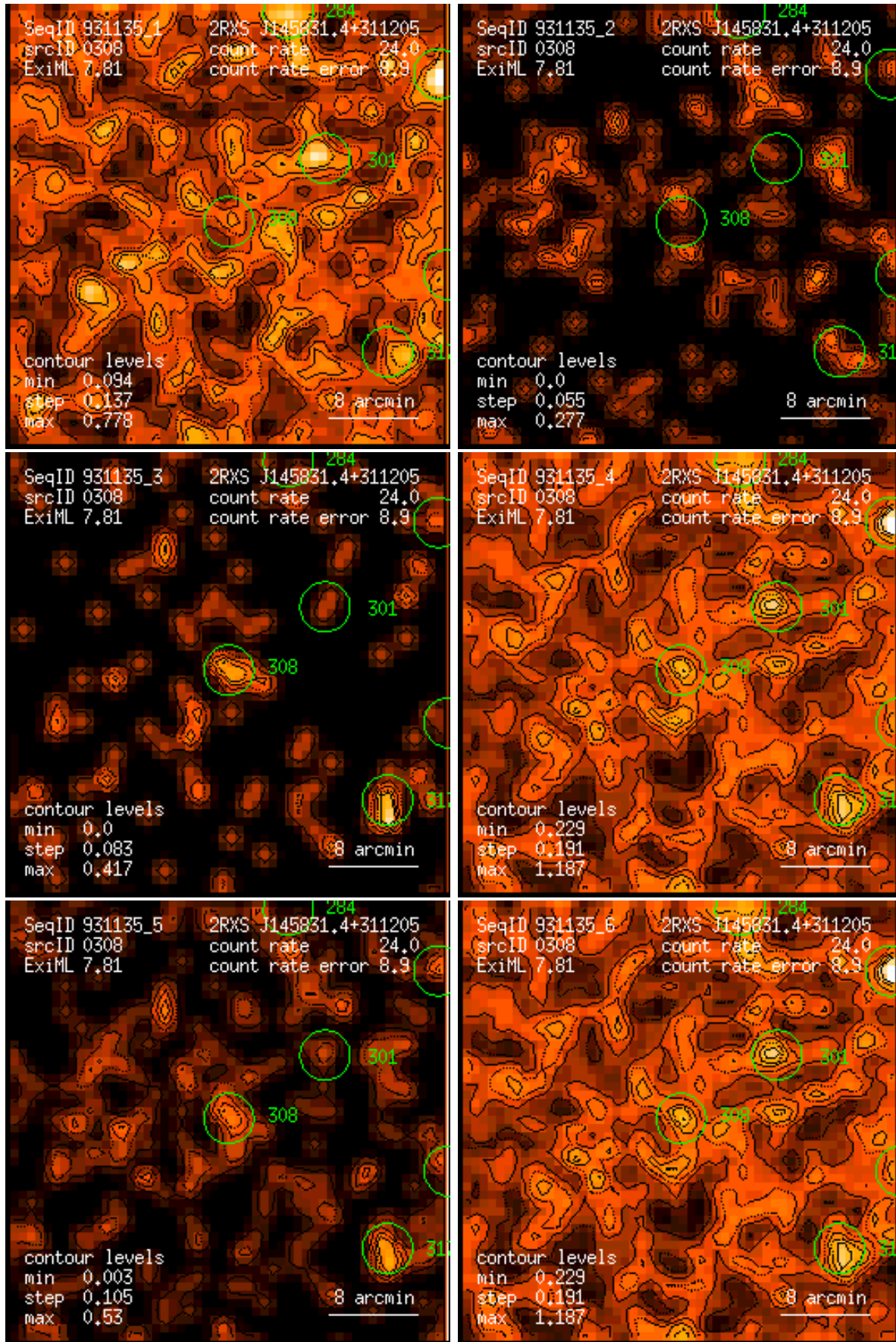
Figure 308: RASS 931135: detection 0308: band rate images, Gaussian filter: (1) PSPC channels 11 – 41, (2) 52 – 90, (3) 91 – 201, (4) 11 – 235, (5) 52 – 201, (6) 11 – 201. Broad band rates in counts/ks. Band rate contour levels in counts/ks/arcmin 2 .
