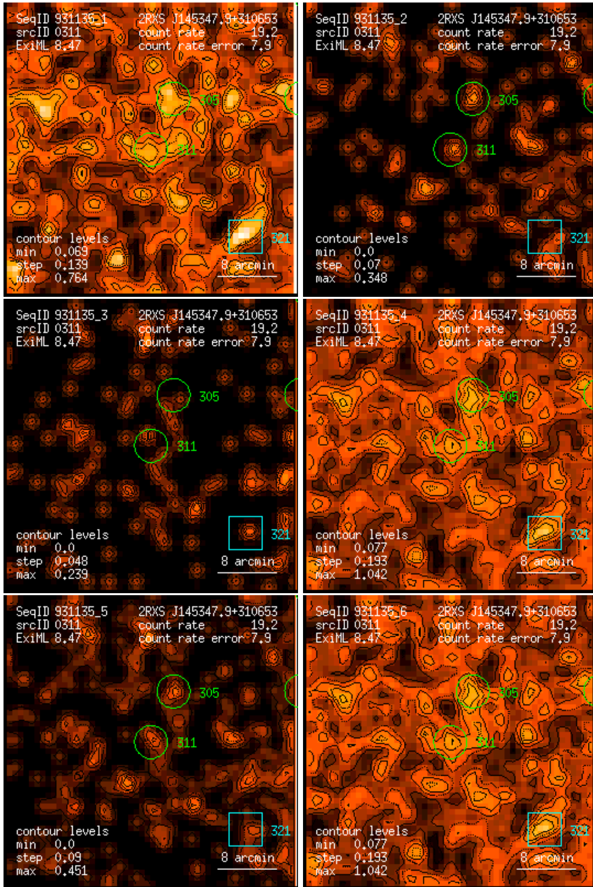
Figure 311: RASS 931135: detection 0311: band rate images, Gaussian filter: (1) PSPC channels 11 – 41, (2) 52 – 90, (3) 91 – 201, (4) 11 – 235, (5) 52 – 201, (6) 11 – 201. Broad band rates in counts/ks. Band rate contour levels in counts/ks/arcmin 2 .
