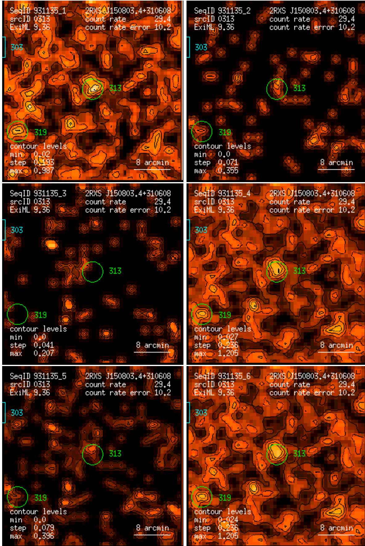
Figure 313: RASS 931135: detection 0313: band rate images, Gaussian filter: (1) PSPC channels 11 – 41, (2) 52 – 90, (3) 91 – 201, (4) 11 – 235, (5) 52 – 201, (6) 11 – 201. Broad band rates in counts/ks. Band rate contour levels in counts/ks/arcmin 2 .
