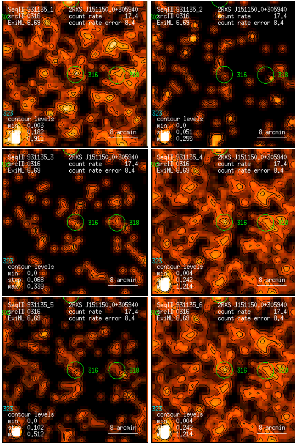
Figure 316: RASS 931135: detection 0316: band rate images, Gaussian filter: (1) PSPC channels 11 – 41, (2) 52 – 90, (3) 91 – 201, (4) 11 – 235, (5) 52 – 201, (6) 11 – 201. Broad band rates in counts/ks. Band rate contour levels in counts/ks/arcmin 2 .
