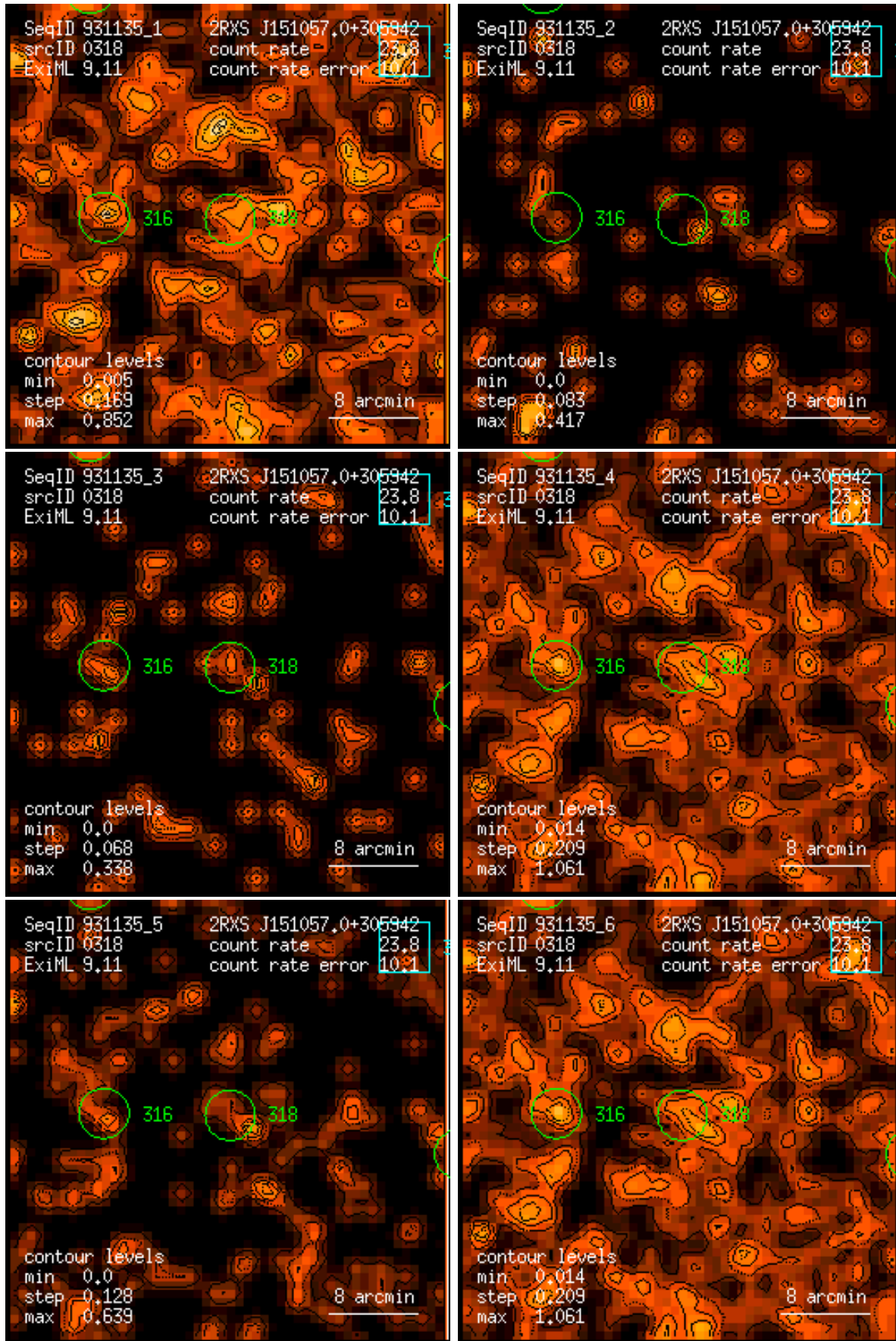
Figure 318: RASS 931135: detection 0318: band rate images, Gaussian filter: (1) PSPC channels 11 – 41, (2) 52 – 90, (3) 91 – 201, (4) 11 – 235, (5) 52 – 201, (6) 11 – 201. Broad band rates in counts/ks. Band rate contour levels in counts/ks/arcmin 2 .
