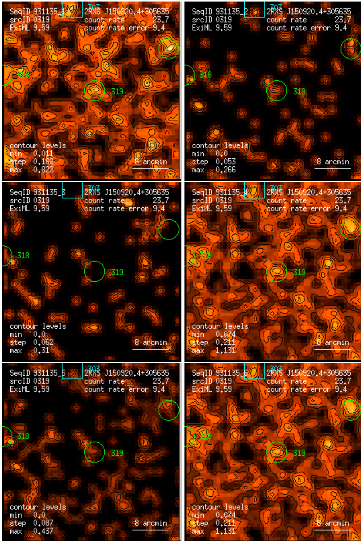
Figure 319: RASS 931135: detection 0319: band rate images, Gaussian filter: (1) PSPC channels 11 – 41, (2) 52 – 90, (3) 91 – 201, (4) 11 – 235, (5) 52 – 201, (6) 11 – 201. Broad band rates in counts/ks. Band rate contour levels in counts/ks/arcmin 2 .
