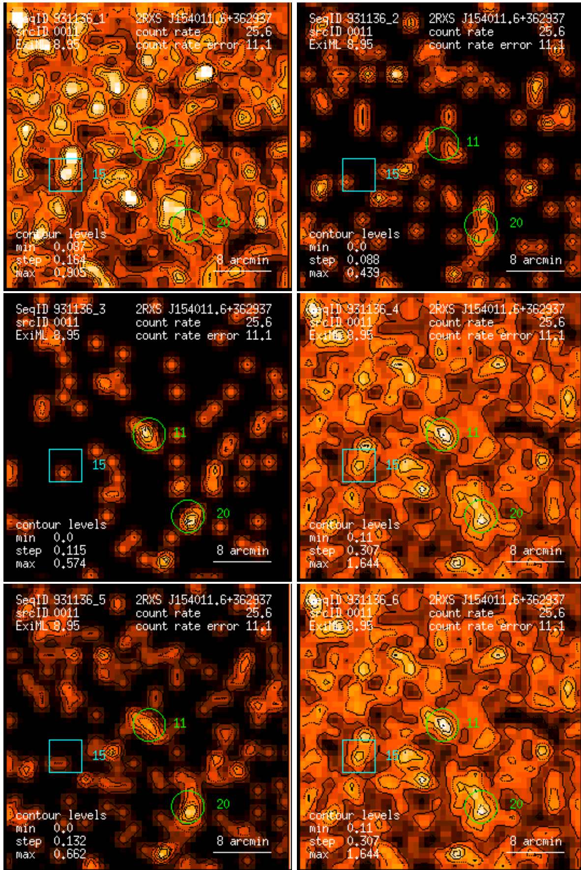
Figure 11: RASS 931136: detection 0011: band rate images, Gaussian filter: (1) PSPC channels 11 – 41, (2) 52 – 90, (3) 91 – 201, (4) 11 – 235, (5) 52 – 201, (6) 11 – 201. Broad band rates in counts/ks. Band rate contour levels in counts/ks/arcmin 2 .
