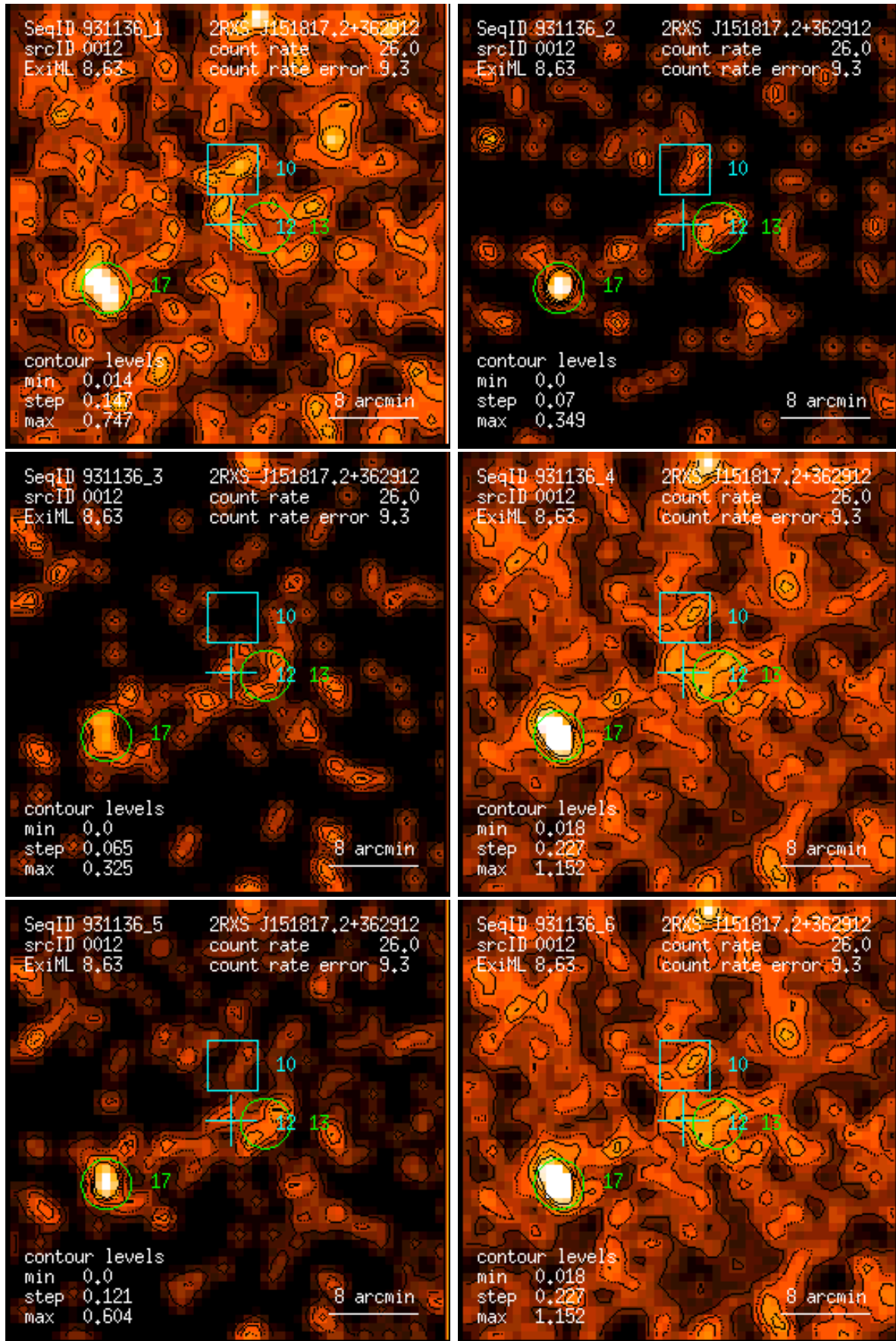
Figure 12: RASS 931136: detection 0012: band rate images, Gaussian filter: (1) PSPC channels 11 – 41, (2) 52 – 90, (3) 91 – 201, (4) 11 – 235, (5) 52 – 201, (6) 11 – 201. Broad band rates in counts/ks. Band rate contour levels in counts/ks/arcmin 2 .
