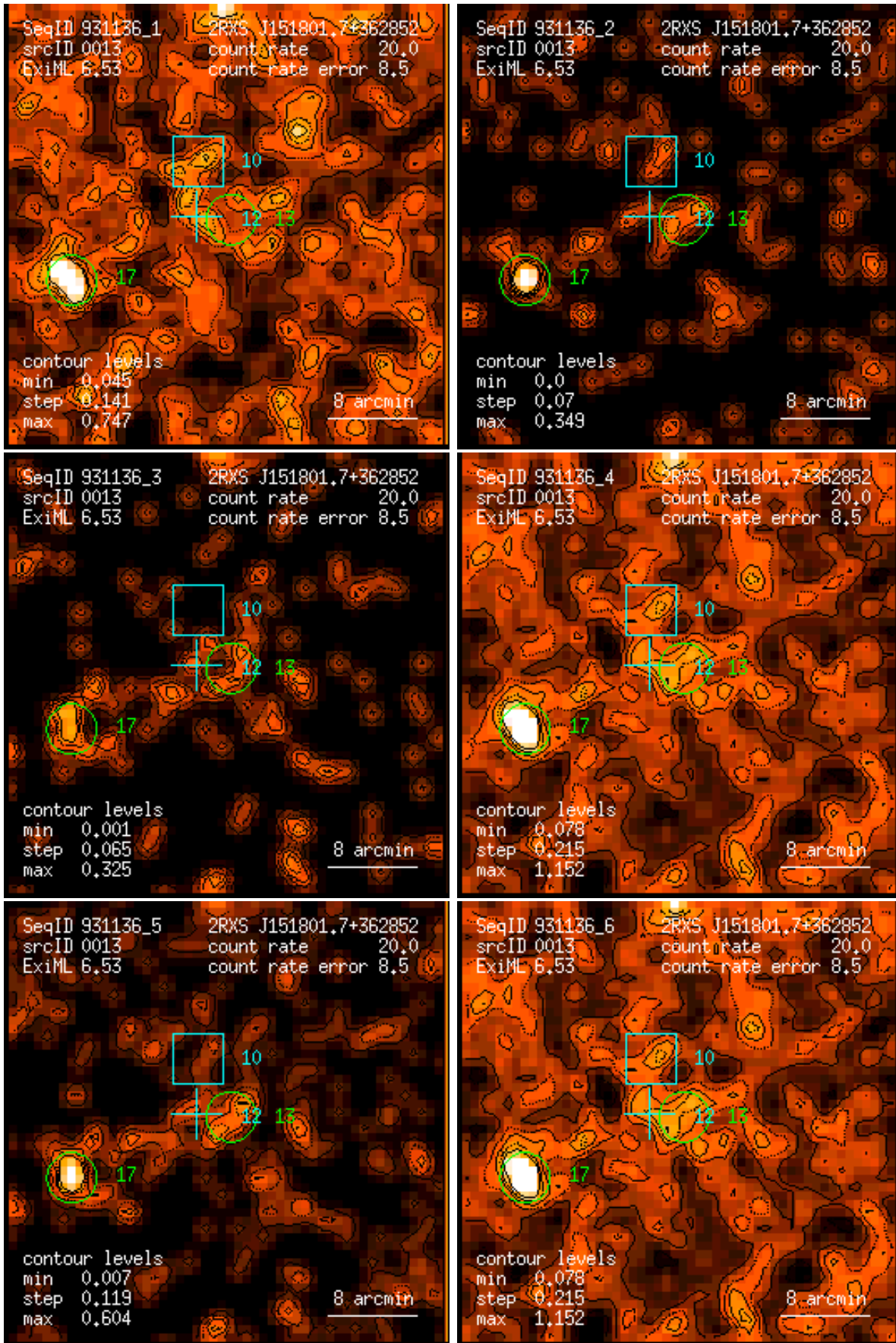
Figure 13: RASS 931136: detection 0013: band rate images, Gaussian filter: (1) PSPC channels 11 – 41, (2) 52 – 90, (3) 91 – 201, (4) 11 – 235, (5) 52 – 201, (6) 11 – 201. Broad band rates in counts/ks. Band rate contour levels in counts/ks/arcmin 2 .
