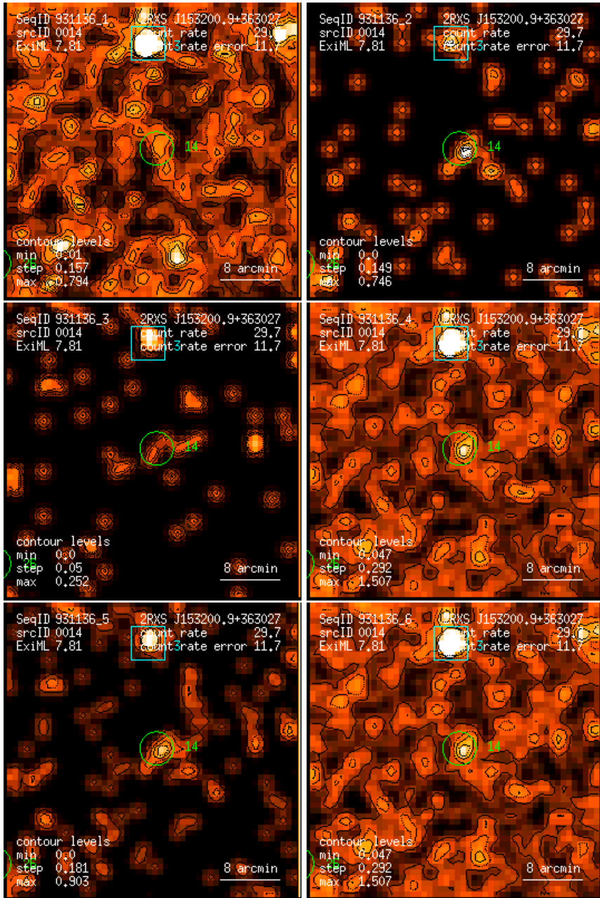
Figure 14: RASS 931136: detection 0014: band rate images, Gaussian filter: (1) PSPC channels 11 – 41, (2) 52 – 90, (3) 91 – 201, (4) 11 – 235, (5) 52 – 201, (6) 11 – 201. Broad band rates in counts/ks. Band rate contour levels in counts/ks/arcmin 2 .
