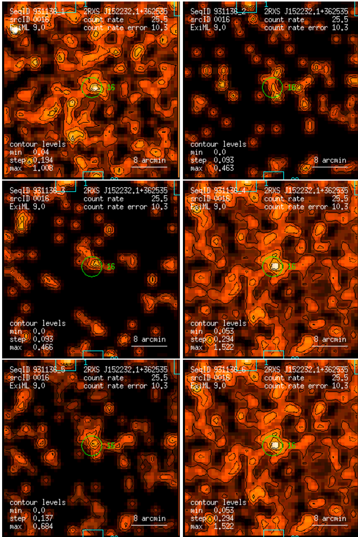
Figure 16: RASS 931136: detection 0016: band rate images, Gaussian filter: (1) PSPC channels 11 – 41, (2) 52 – 90, (3) 91 – 201, (4) 11 – 235, (5) 52 – 201, (6) 11 – 201. Broad band rates in counts/ks. Band rate contour levels in counts/ks/arcmin 2 .
