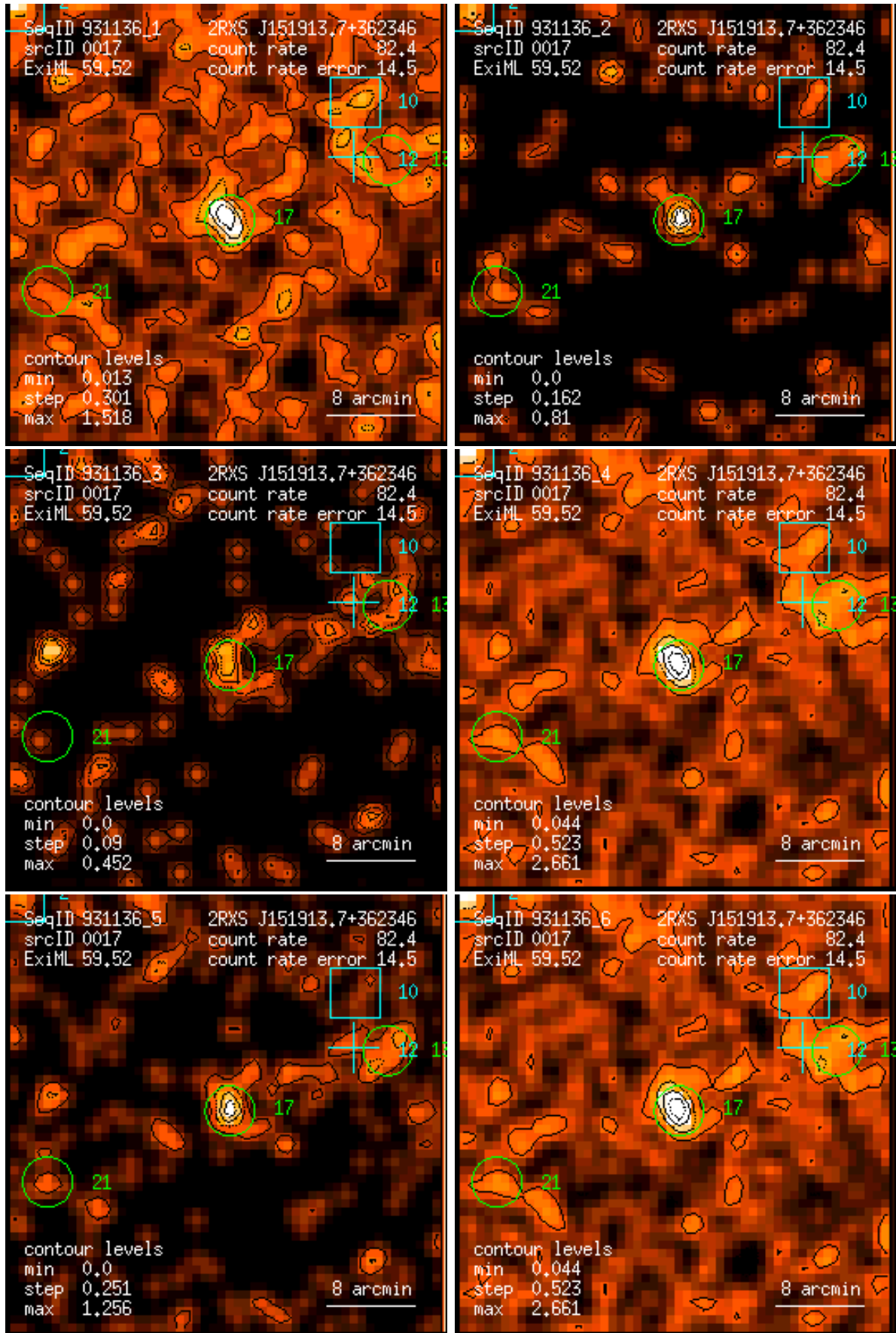
Figure 17: RASS 931136: detection 0017: band rate images, Gaussian filter: (1) PSPC channels 11 – 41, (2) 52 – 90, (3) 91 – 201, (4) 11 – 235, (5) 52 – 201, (6) 11 – 201. Broad band rates in counts/ks. Band rate contour levels in counts/ks/arcmin 2 .
