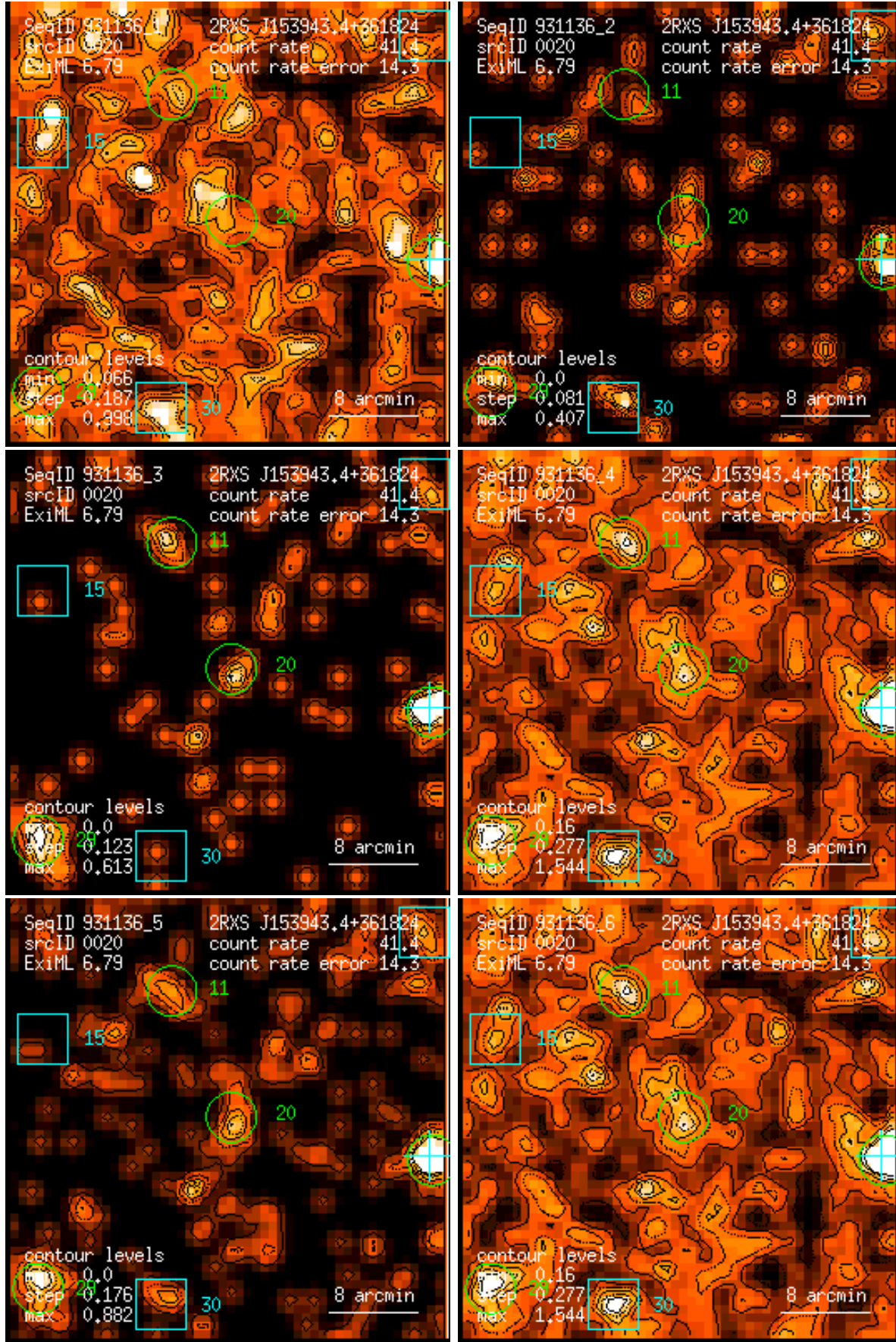
Figure 20: RASS 931136: detection 0020: band rate images, Gaussian filter: (1) PSPC channels 11 – 41, (2) 52 – 90, (3) 91 – 201, (4) 11 – 235, (5) 52 – 201, (6) 11 – 201. Broad band rates in counts/ks. Band rate contour levels in counts/ks/arcmin 2 .
