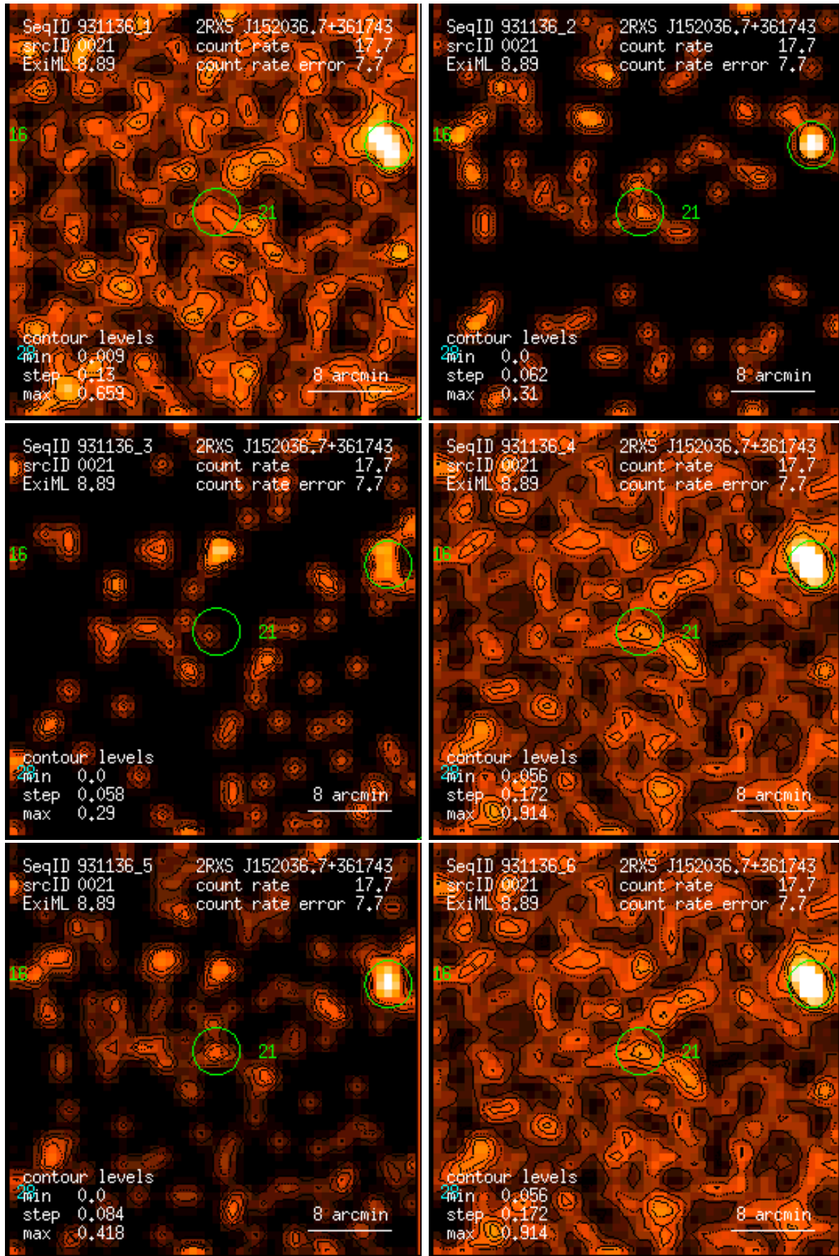
Figure 21: RASS 931136: detection 0021: band rate images, Gaussian filter: (1) PSPC channels 11 – 41, (2) 52 – 90, (3) 91 – 201, (4) 11 – 235, (5) 52 – 201, (6) 11 – 201. Broad band rates in counts/ks. Band rate contour levels in counts/ks/arcmin 2 .
