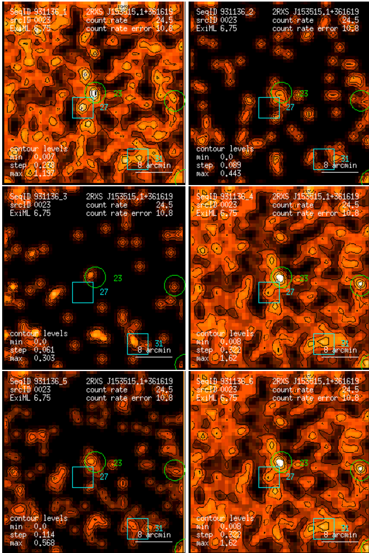
Figure 23: RASS 931136: detection 0023: band rate images, Gaussian filter: (1) PSPC channels 11 – 41, (2) 52 – 90, (3) 91 – 201, (4) 11 – 235, (5) 52 – 201, (6) 11 – 201. Broad band rates in counts/ks. Band rate contour levels in counts/ks/arcmin 2 .
