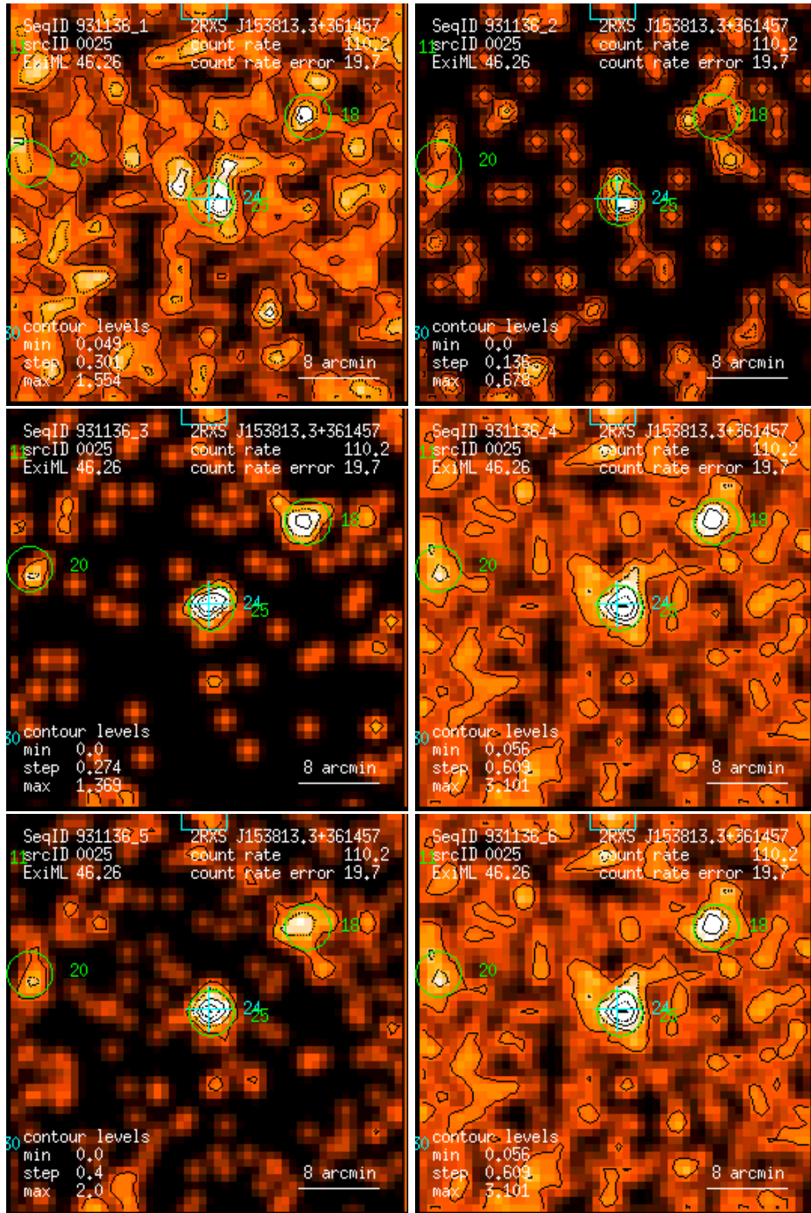
Figure 25: RASS 931136: detection 0025: band rate images, Gaussian filter: (1) PSPC channels 11 – 41, (2) 52 – 90, (3) 91 – 201, (4) 11 – 235, (5) 52 – 201, (6) 11 – 201. Broad band rates in counts/ks. Band rate contour levels in counts/ks/arcmin 2 .
