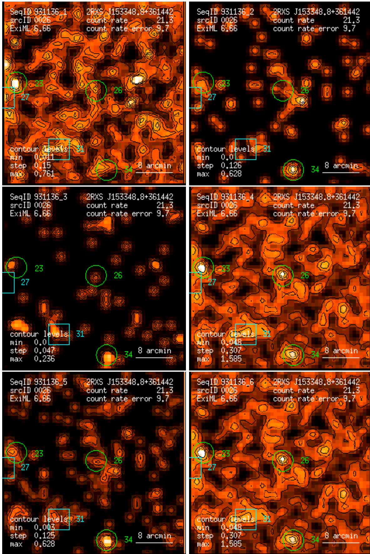
Figure 26: RASS 931136: detection 0026: band rate images, Gaussian filter: (1) PSPC channels 11 – 41, (2) 52 – 90, (3) 91 – 201, (4) 11 – 235, (5) 52 – 201, (6) 11 – 201. Broad band rates in counts/ks. Band rate contour levels in counts/ks/arcmin 2 .
