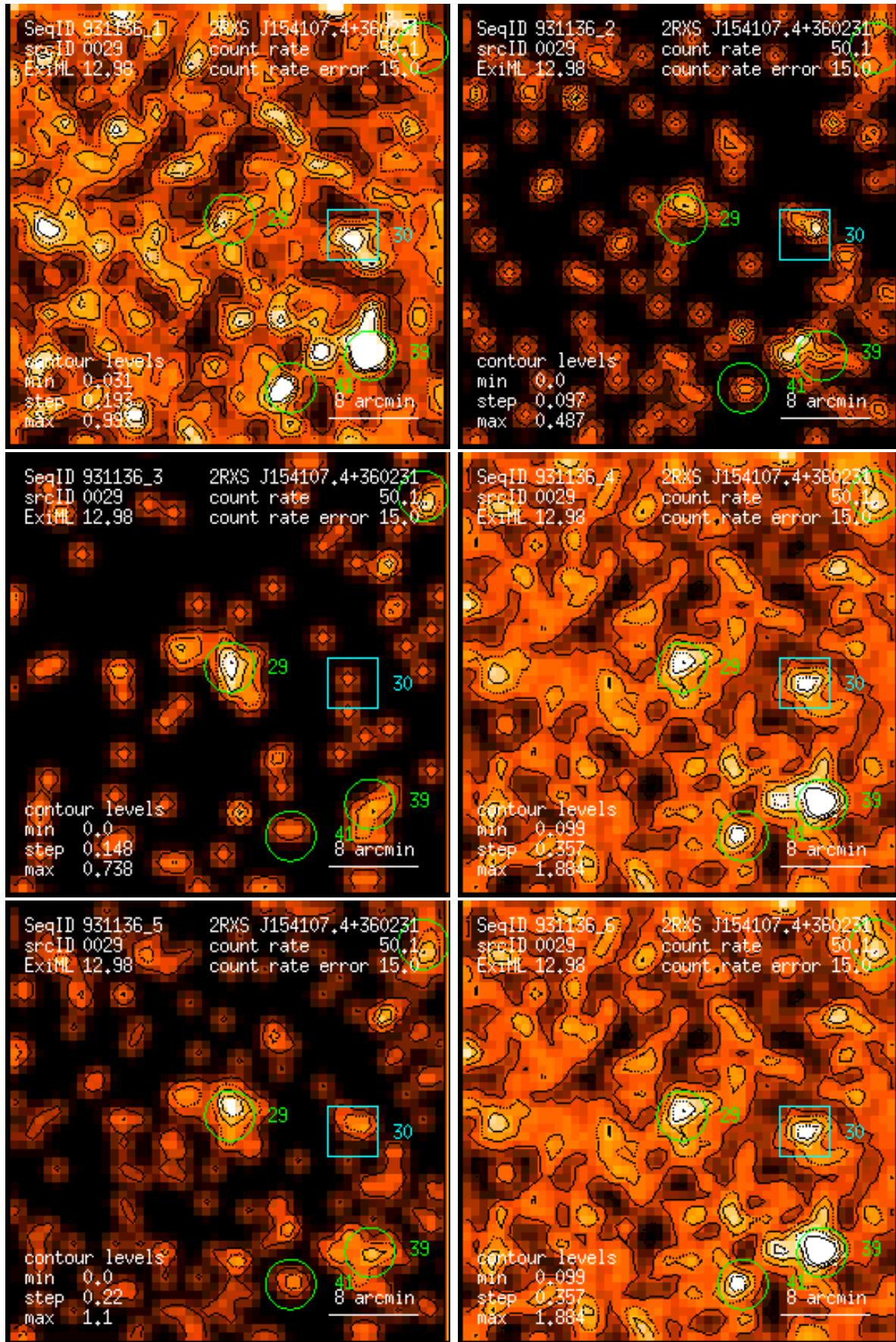
Figure 29: RASS 931136: detection 0029: band rate images, Gaussian filter: (1) PSPC channels 11 – 41, (2) 52 – 90, (3) 91 – 201, (4) 11 – 235, (5) 52 – 201, (6) 11 – 201. Broad band rates in counts/ks. Band rate contour levels in counts/ks/arcmin 2 .
