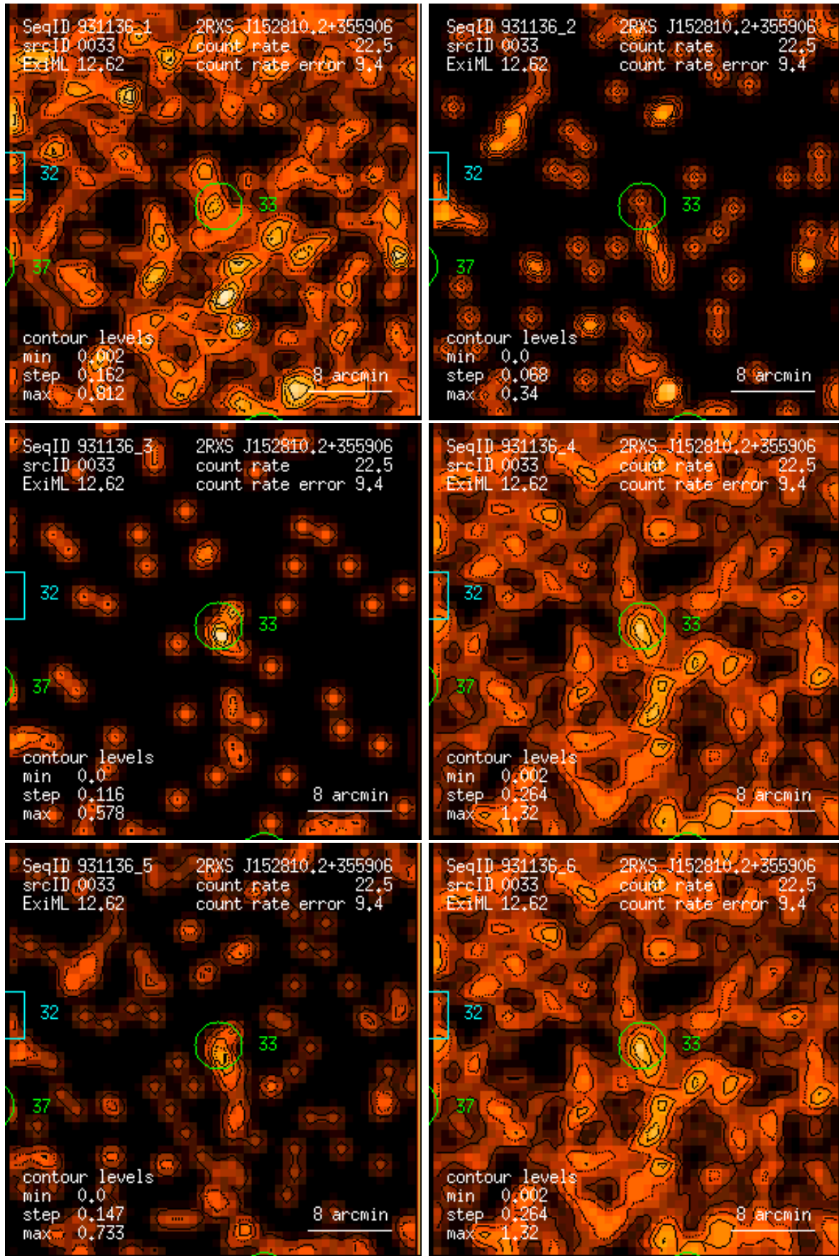
Figure 33: RASS 931136: detection 0033: band rate images, Gaussian filter: (1) PSPC channels 11 – 41, (2) 52 – 90, (3) 91 – 201, (4) 11 – 235, (5) 52 – 201, (6) 11 – 201. Broad band rates in counts/ks. Band rate contour levels in counts/ks/arcmin 2 .
