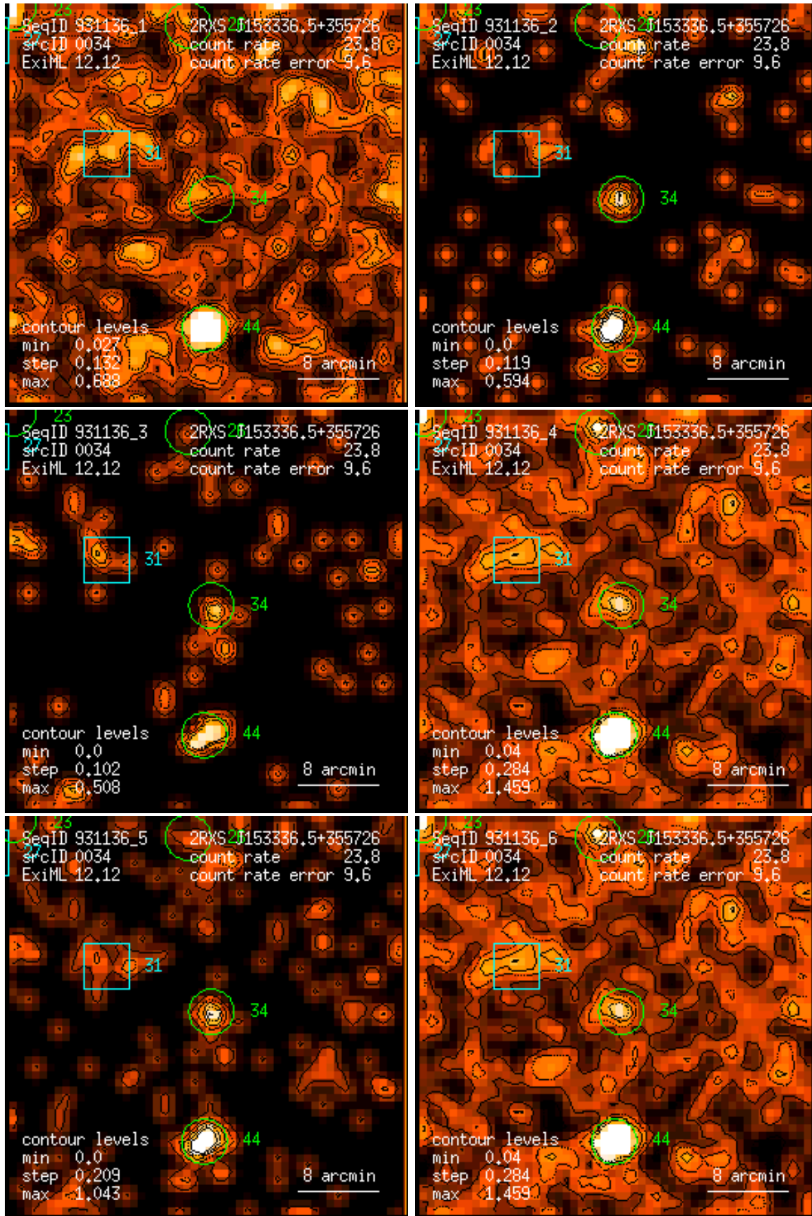
Figure 34: RASS 931136: detection 0034: band rate images, Gaussian filter: (1) PSPC channels 11 – 41, (2) 52 – 90, (3) 91 – 201, (4) 11 – 235, (5) 52 – 201, (6) 11 – 201. Broad band rates in counts/ks. Band rate contour levels in counts/ks/arcmin 2 .
