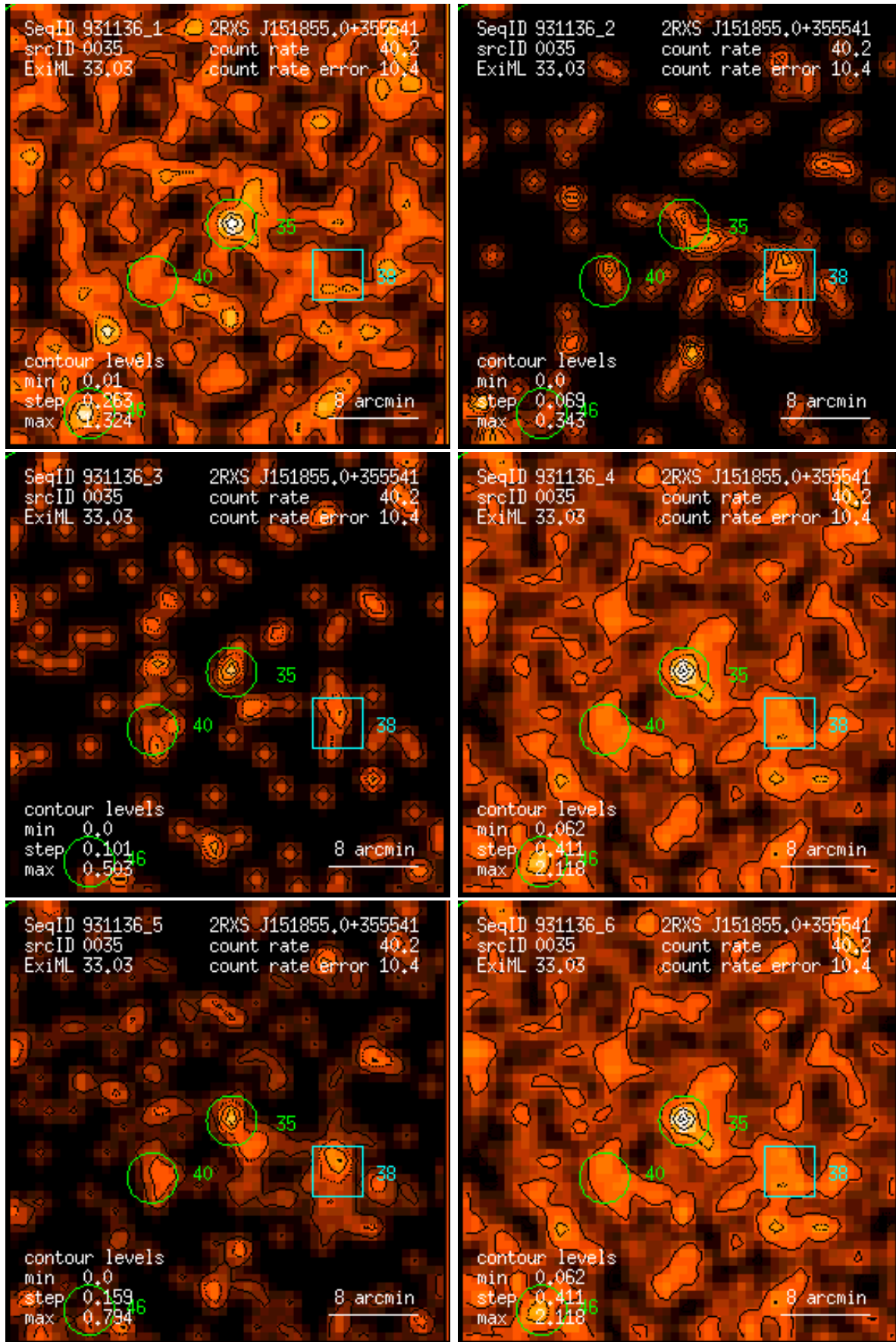
Figure 35: RASS 931136: detection 0035: band rate images, Gaussian filter: (1) PSPC channels 11 – 41, (2) 52 – 90, (3) 91 – 201, (4) 11 – 235, (5) 52 – 201, (6) 11 – 201. Broad band rates in counts/ks. Band rate contour levels in counts/ks/arcmin 2 .
