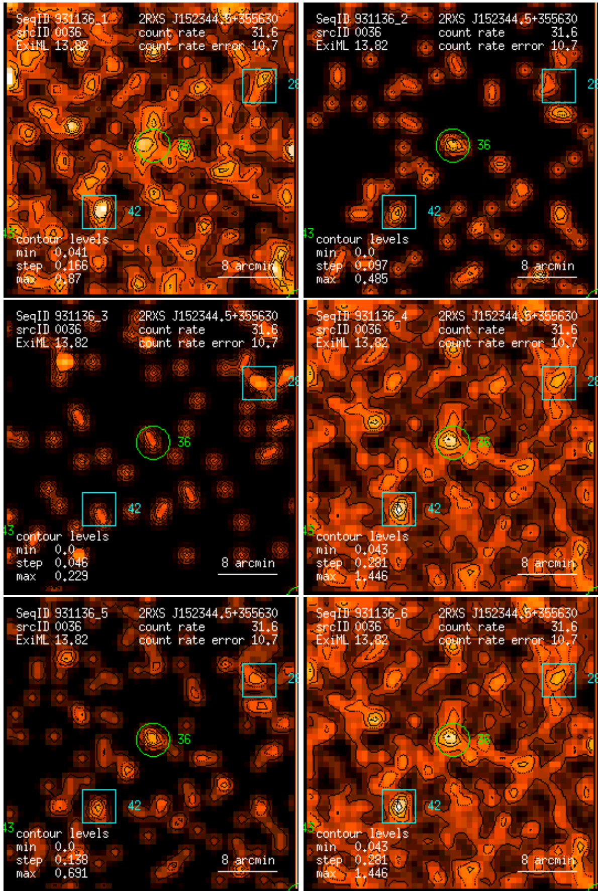
Figure 36: RASS 931136: detection 0036: band rate images, Gaussian filter: (1) PSPC channels 11 – 41, (2) 52 – 90, (3) 91 – 201, (4) 11 – 235, (5) 52 – 201, (6) 11 – 201. Broad band rates in counts/ks. Band rate contour levels in counts/ks/arcmin 2 .
