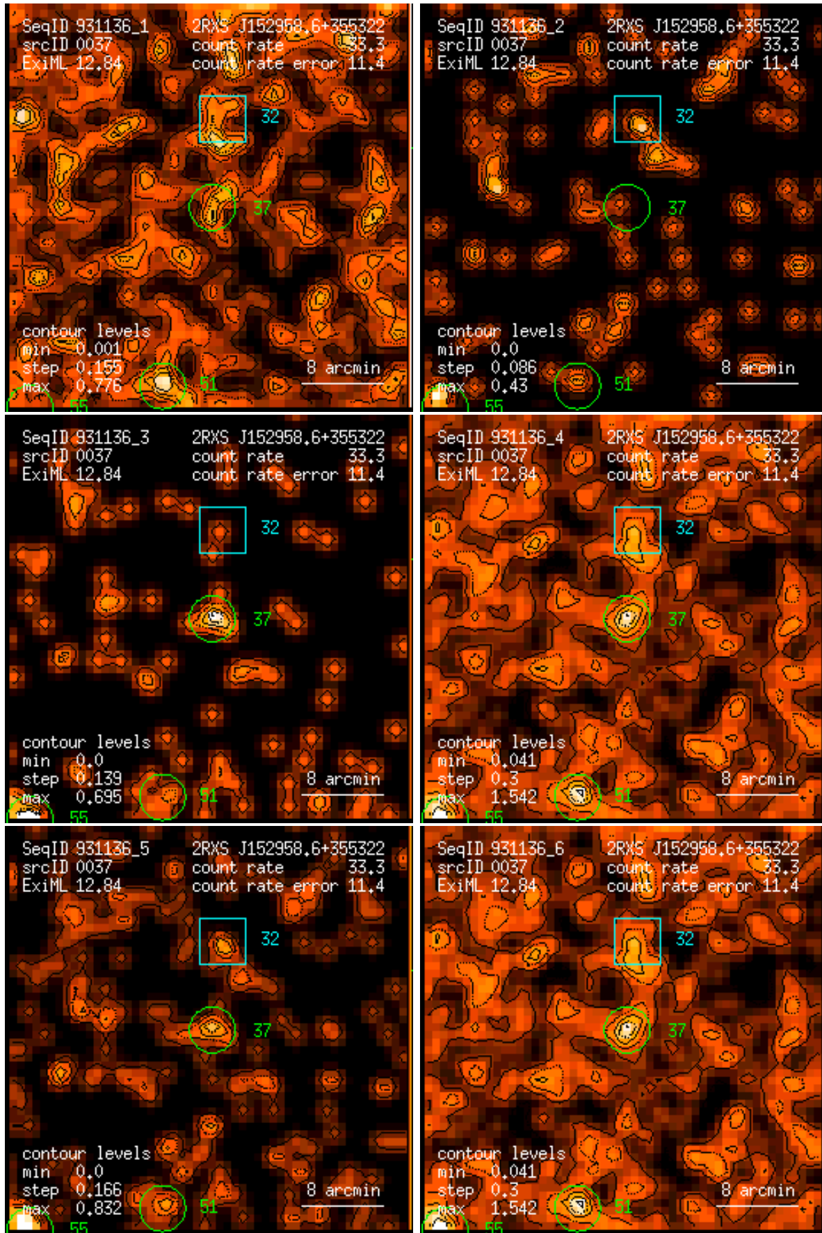
Figure 37: RASS 931136: detection 0037: band rate images, Gaussian filter: (1) PSPC channels 11 – 41, (2) 52 – 90, (3) 91 – 201, (4) 11 – 235, (5) 52 – 201, (6) 11 – 201. Broad band rates in counts/ks. Band rate contour levels in counts/ks/arcmin 2 .
