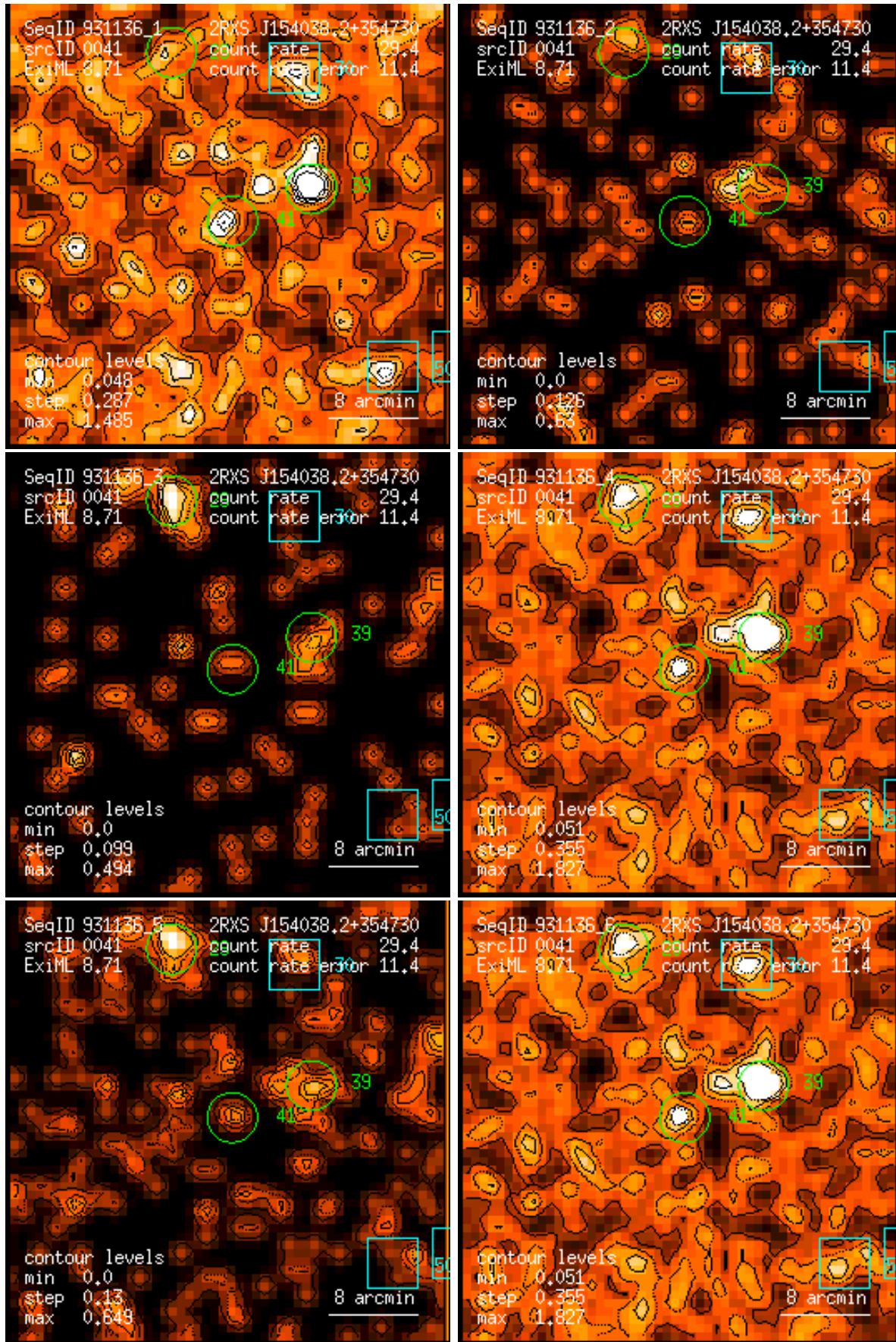
Figure 41: RASS 931136: detection 0041: band rate images, Gaussian filter: (1) PSPC channels 11 – 41, (2) 52 – 90, (3) 91 – 201, (4) 11 – 235, (5) 52 – 201, (6) 11 – 201. Broad band rates in counts/ks. Band rate contour levels in counts/ks/arcmin 2 .
