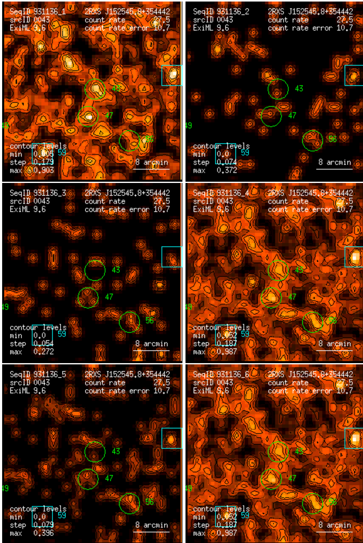
Figure 43: RASS 931136: detection 0043: band rate images, Gaussian filter: (1) PSPC channels 11 – 41, (2) 52 – 90, (3) 91 – 201, (4) 11 – 235, (5) 52 – 201, (6) 11 – 201. Broad band rates in counts/ks. Band rate contour levels in counts/ks/arcmin 2 .
