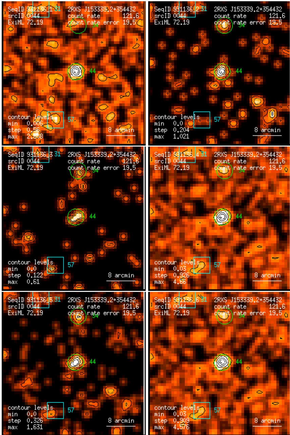
Figure 44: RASS 931136: detection 0044: band rate images, Gaussian filter: (1) PSPC channels 11 – 41, (2) 52 – 90, (3) 91 – 201, (4) 11 – 235, (5) 52 – 201, (6) 11 – 201. Broad band rates in counts/ks. Band rate contour levels in counts/ks/arcmin 2 .
